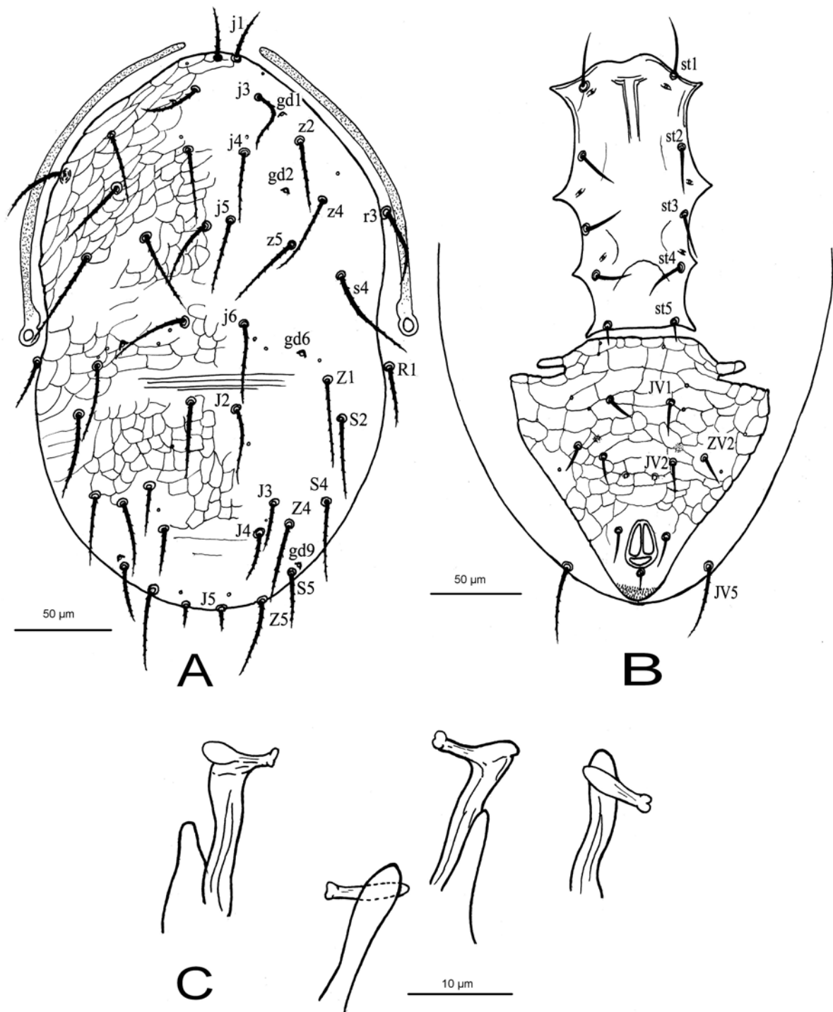
FIGURE 3: Ragusaseius ferraguti n. g., n. sp.. Male; (A) – Dorsal idiosoma; (B) – Ventral idiosoma; (C) – Spermatodactyl.
