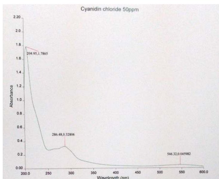
Fig 11. UV-visible spectrum of cyanidin chloride at 50 \mu\text{g mL}^{-1} .
