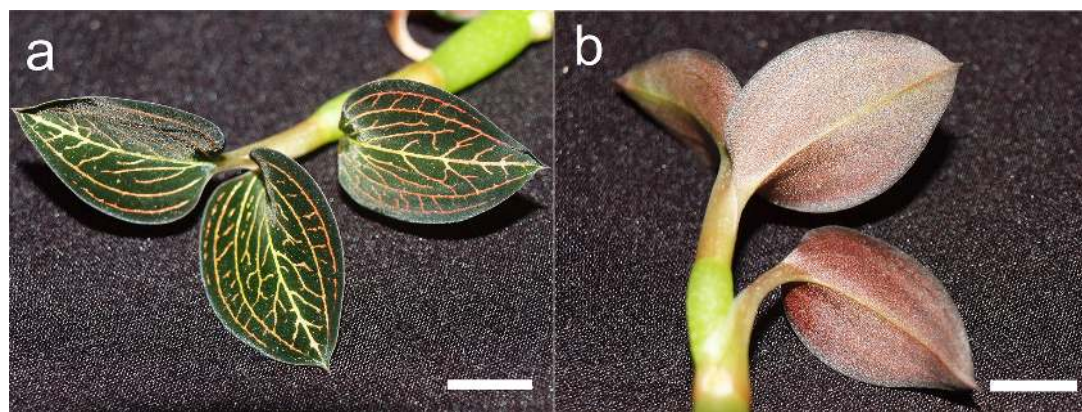
Fig 3. A mature L. discolor plant. Leaves of the plant displayed a dark green adaxial surface laced with golden veins, and a red abaxial layer. Bar = 1 cm.
