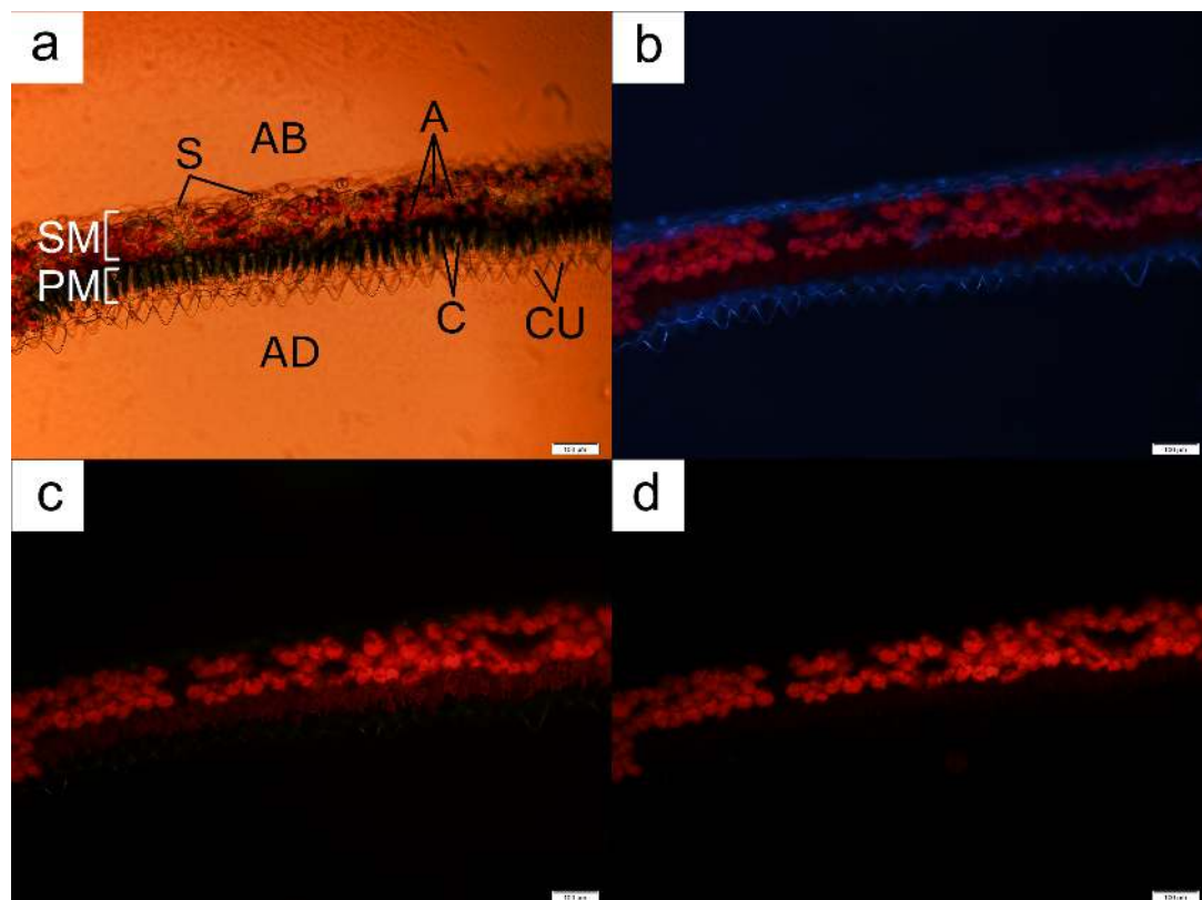
Fig 9. A leaf cross-section from L. discolor displaying cells with multiple anthocyanic layers. The arrangement of cells containing chloroplasts (C) and anthocyanins (A) were observed under brightfield microscopy (a), UV rays (b), blue light (c) and green light (d). AB = abaxial; AD = adaxial; CU = cuticle; PM = palisade mesophyll; S = stoma; SM = spongy mesophyll. Bar = 100 \mu m.
