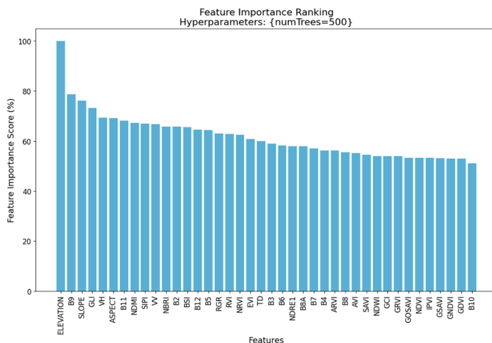
Figure 6. Feature importance based on Dataset 2 for the RF_3 hyperparameter.
