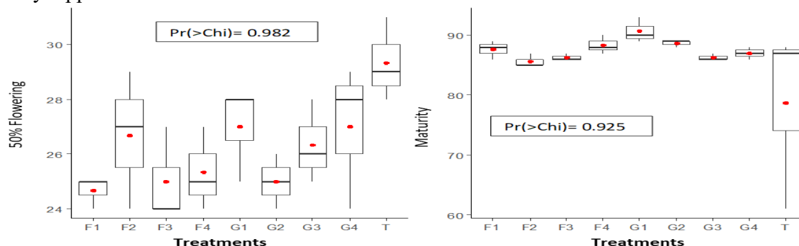
Figure 8. Cycle variation (50% flowering and maturity) according to treatments.
