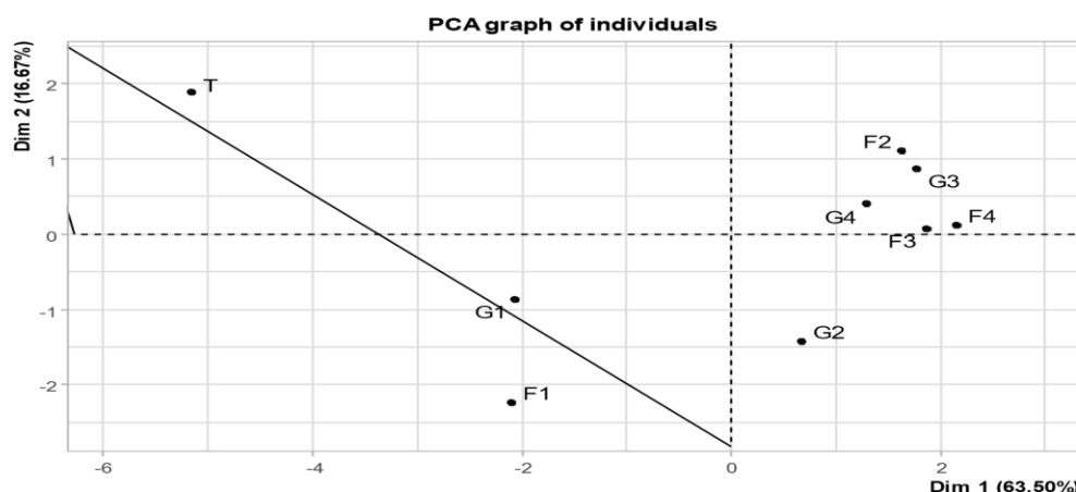
Figure 12. Principal component plot of the different treatments
