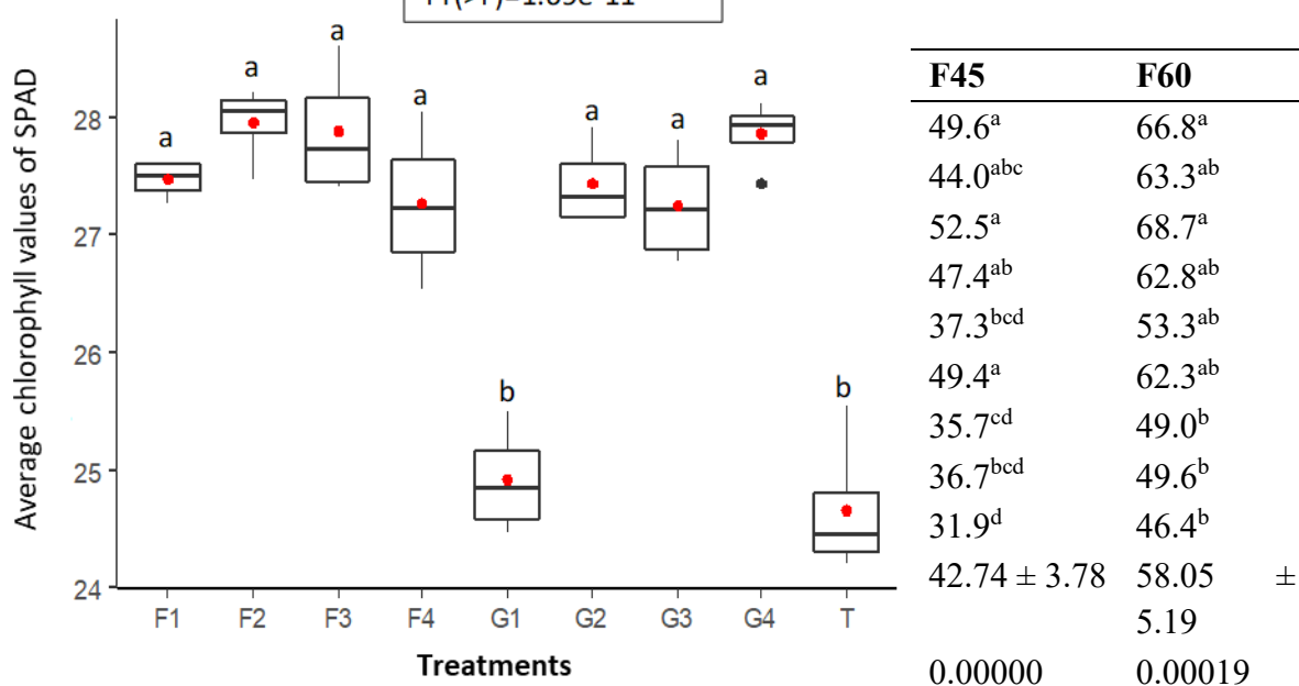
Figure 7. Variation in average chlorophyll values of SPAD as a function of treatments.
