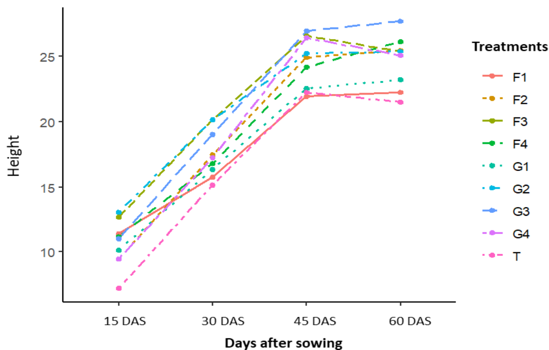
Figure 3. Evolution of the height (cm) of the plants as a function of time.
