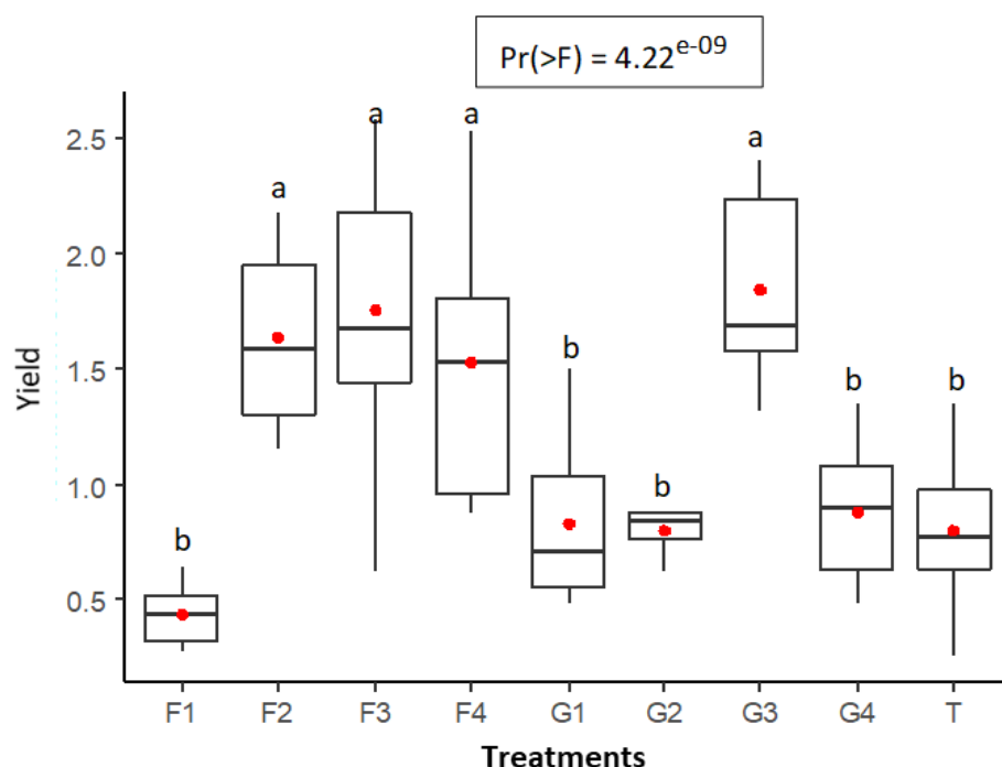
Figure 9. Variation in seed yield by treatment. influenced by an early maturity and high chlorophyll values. Treatments G1 and F1 were very particular, because as for the control (T) and G2, they were very opposed to the
