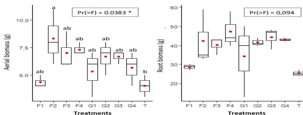
Figure 10. Variation in dry biomass (aerial and root) between treatments.
