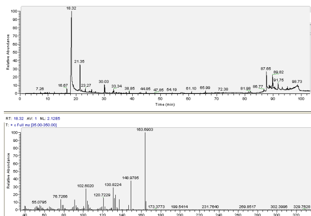
Fig. 2 GC-MS chromatogram of SC-CO 2 extract of bay leaves obtained at 55°C, 512 bar and 60 min extraction time
