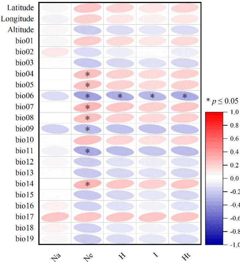
FIGURE 2 Correlation heat map between genetic diversity index and geographical and bioclimatic variables. * indicate significant correlation at the p \leq 0.05 level.
