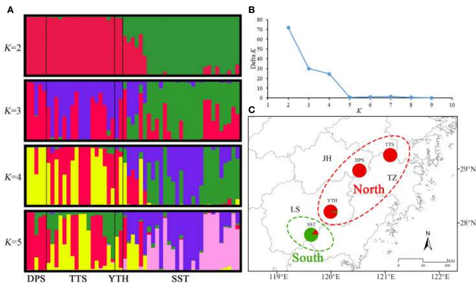
FIGURE 3 Bayesian clustering results of C. tientaiensis . (A) Composition of genetic branches for each individual when K=2, 3, 4, and 5 ; (B) Delta K ; (C) Bayesian clustering results when K=2 . JH, Jinhua city; LS, Lishui city; TZ, Taizhou city; TTS, Tiantai Mountain, Taizhou city; DPS, Dapan Mountain, Jinhua city; YTH, Yangtianhe, Lishui city; SST, Shangshantou, Lishui city.
