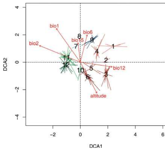
Figure 3. DCA ordination of forb steppe communities in the Pamir-Alai Mountains. The different colors refer to alliances: red – Ligulario thomsonii - Geranium regelii , blue – Artemision dracunculi and green – Poa alpinae - Bistortion ellipticae . Numbers on the ordination refer to centroids of clusters (see Figure 2 and Syntaxonomic synopsis).
