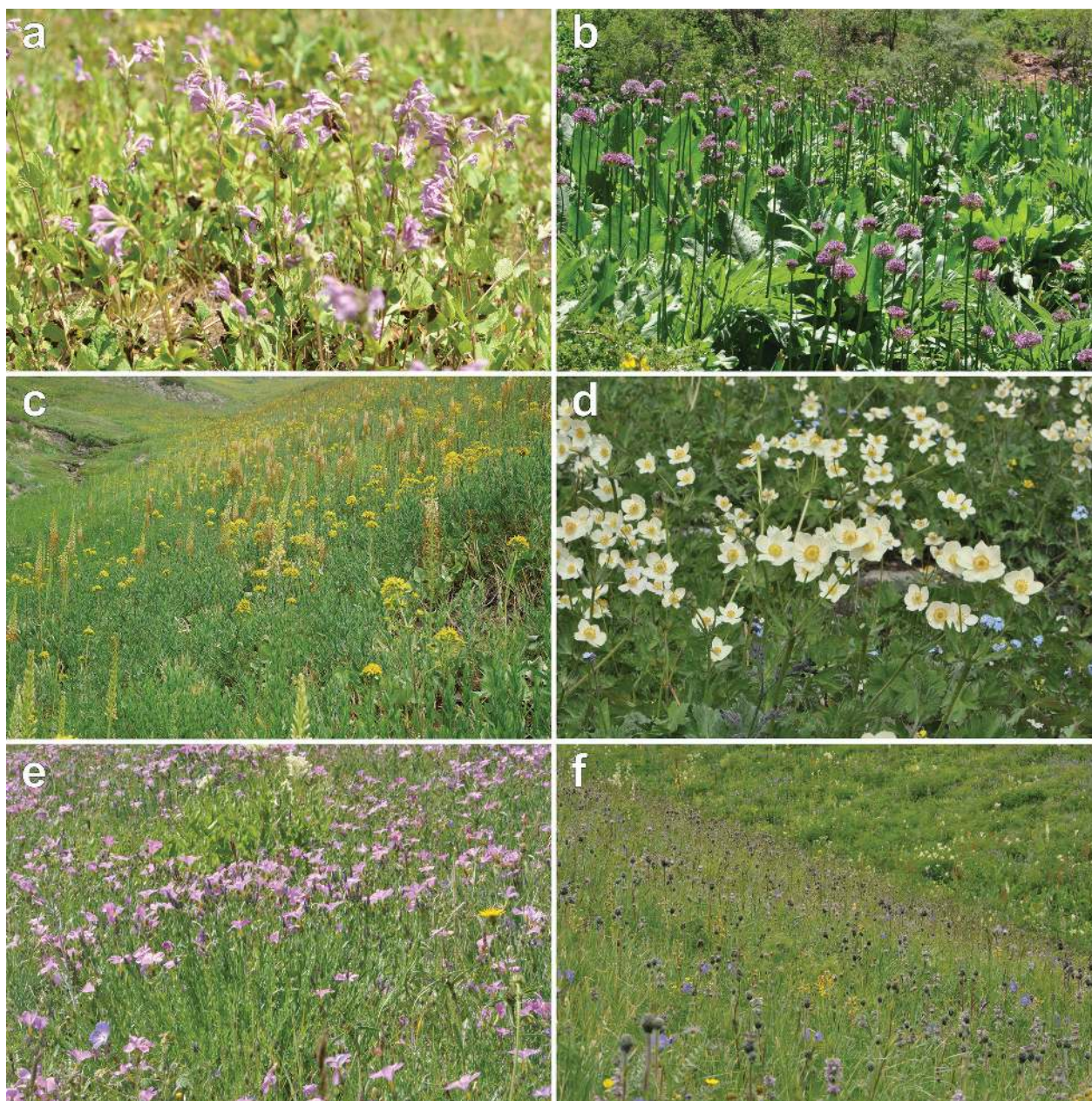
Figure 8. Photographs of mesophilous steppic pastures of the subalpine belt and mesic grasslands of the alpine belt belonging to: a – community of Dracocephalum formosum in the Zeravshan Mountains; b – community of Allium giganteum near the Kosh-Ob village in Vakhsh Mountains; c – Erigeronto seravschanici - Eremuretum hissarici near the Anzob Pass, Hissar Mts; d – Poo alpinae - Swertietum graciliflorae near the Anzob Pass, Hissar Mts; e – Astragalo alpini - Linetum olgae in the Fann Mountains; f – Ligularia alpigenae - Solenanthes karategini near the Koshtegirmen village, the Peter the First Mountains (pictures a, b, d, e, f were taken by A. Nowak and c by S. Świerszcz).
