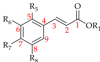
Figure 14. Basic structure of hydroxycinnamic acid and its derivatives (HCADs) (see 90–109 in Table 9).
