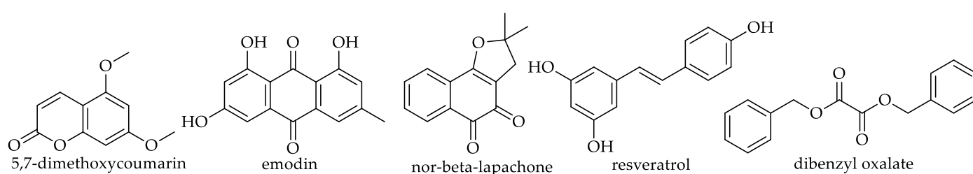
Figure 21. Structure of 5,7-dimethoxycoumarin (157, Table 15), emodin (158, Table 15), nor-β-lapachone (159, Table 15), resveratrol, a stilbene (160, Table 15), and dibenzyl oxalate, an oxalate ester (161, Table 15) reported in honeys.
