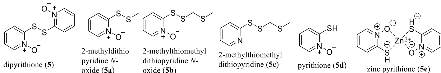
Figure 4. Structures of the thiopyridine dipyrithione ( 5 ) isolated from the Lao plant, Marsypopetalum modestum , and its analogues ( 5a–5e ) (Elkington et al. 2014b, O'Donnell et al. 2009, Krejčová et al. 2014, Liu et al. 2008, Srivastava et al. 2015, Tailler et al. 2012).
