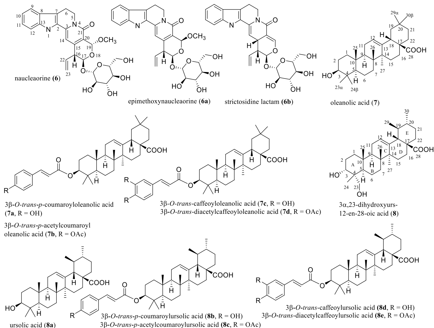
Figure 5. Structures of the alkaloid naucleaorine ( 6 ) and its analogues ( 6a and 6b ) and the triterpenoids oleanolic acid ( 7 ) and 3α,23-dihydroxyurs-12-en-28-oic acid ( 8 ) isolated from the Lao plant, Nauclea orientalis , and selected derivatives, 7a–7d of 7 and 8a–8e of 8 (He et al. 2005, Tanachatchairatana et al. 2008).
