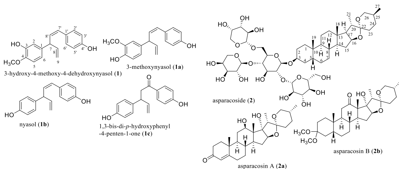
Figure 1. Structures of the norlignan 3-hydroxy-4-methoxy-4-dehydroxyynyasol ( 1 ) and its analogues ( 1a-1c ) and the steroid asparacoside ( 2 ) and its analogues ( 2a and 2b ) isolated from the roots of Asparagus cochinchinensis collected in Laos. Zhang et al. (2004).
