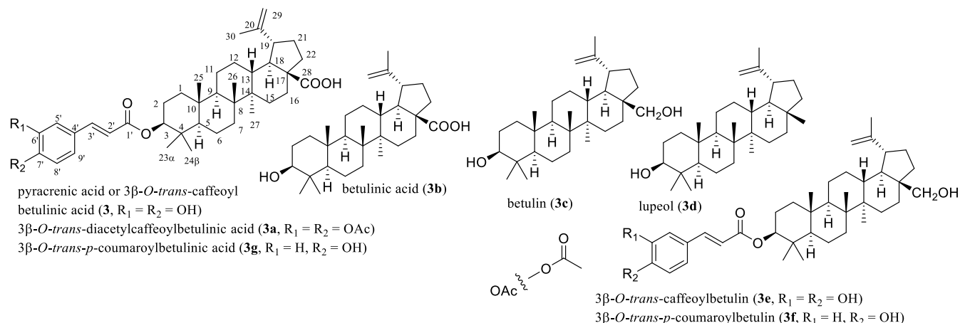
Figure 2. Structures of the triterpenoid pyracrenic acid (3β- O - trans -caffeoyl betulinic acid, 3 ) and betulinic acid ( 3b ) isolated from the Lao plant, Diospyros quaesita , and of selected derivatives 3a and 3c–3g . Lomchid et al. (2017), Ma et al. (2008), and Shi et al. (2014).
