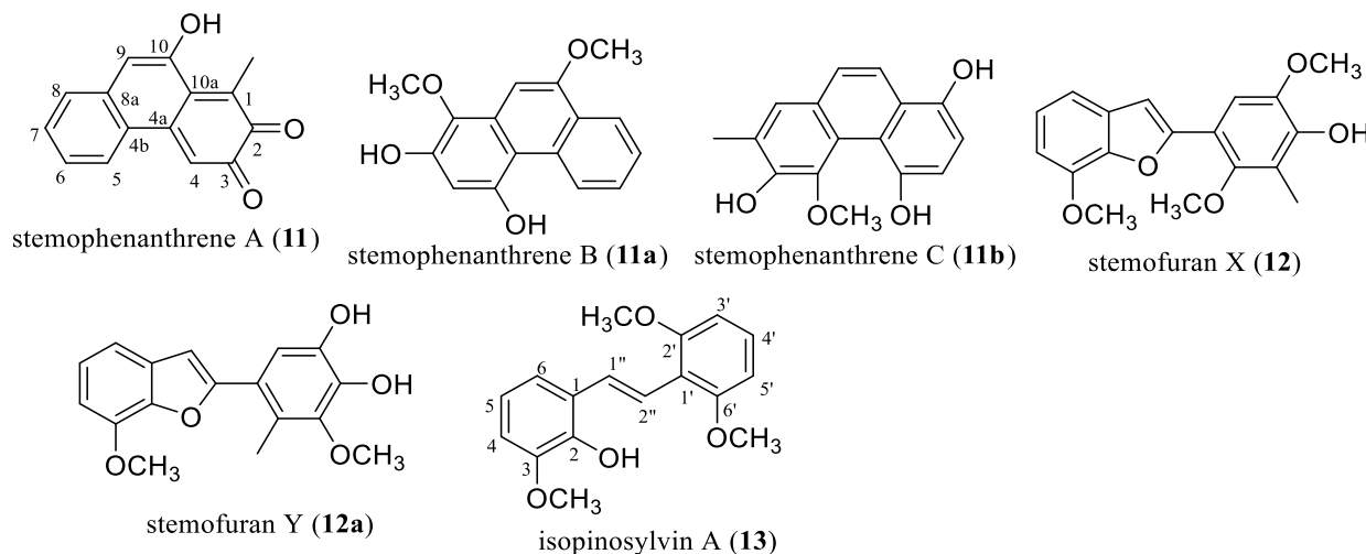
Figure 7. Structures of the phenanthrene stemophenanthrene A ( 11 ) and its analogues ( 11a and 11b ) and the stilbenoids stemofuran Y ( 12a ) and isopinosylvin A ( 13 ) isolated from Stemona tuberosa , as well stemofuran X ( 12 ) isolated from Stemona pierrei , collected in Laos (Khamko et al., 2013; Quang et al., 2014).
