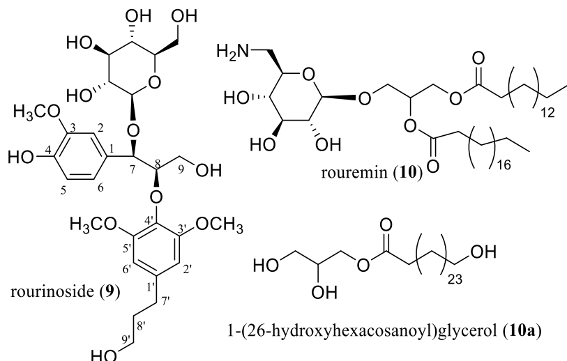
Figure 6. Structures of the lignan rourinoside ( 9 ) and the glycerol ester rouremin ( 10 ) and its analogue ( 10a ) isolated from Rourea minor collected in Laos (He et al., 2006).
