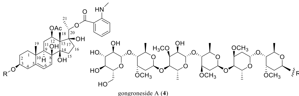
Figure 3. Structure of the steroid glycoside gongroneside A (4) isolated from the Lao plant, Gongronema napalense . Libman et al. (2008).
