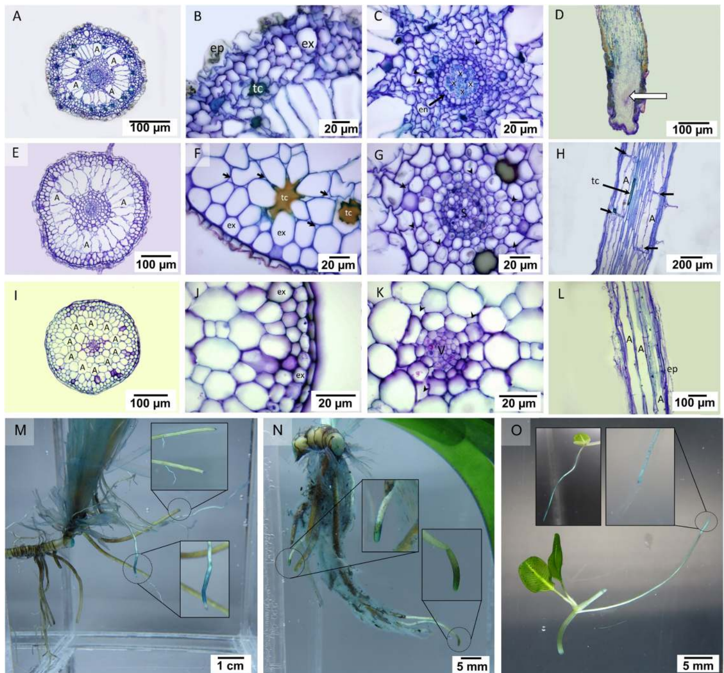
Figure 2 Root anatomical characteristics and localization of oxygen loss. Root anatomical characteristics of seagrasses. (A–D) Cymodocea rotundata , (E–H) Thalassia hemprichii and (I–L) Halophila ovalis and their localization of oxygen loss (M–O): (A) Transverse section of C. rotundata root. (B) The exodermis layers in the outer cortex. (C) The inner cortex with intercellular space (arrow head). (D) Root tip (E) Transverse section of T. hemprichii root. (F) The outer cortex with intercellular space (arrow). (G) Stele and the inner cortex with intercellular space (arrow head). (H) Lacunal diaphragm in the root (arrow). (I) Transverse section of H. ovalis root. (J) Exodermis layers in the outer cortex (K) Stele and inner cortex with intercellular space (arrow head) (L) Diaphragm-free air lacunae root. (M) Cymodocea rotundata root with ROL detected (blue staining) at the root tip. The younger root (lower inset) showed higher oxidation than the older root (upper inset). (N) Thalassia hemprichii root with ROL detected at the root tip. The left inset shows the younger root, and the right inset shows the older root. (O) Oxidized root tip of the second youngest ramet (right inset) and the apical ramet (left inset) of Halophila ovalis . Scale bars: 100 \mu m (A, D, E, I, L); 20 \mu m (B, C, F, G, J, K); 200 \mu m (H); 1 cm (M); 5 mm (N, O) A, Air lacuna; ep, epidermis; en, endodermis; ex, exodermis; s, stele; tc, tanniferous cell; x, xylem; v, vascular tissue.
