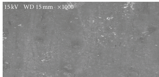
FIGURE 12: SEM Photograph of mild steel immersed in 1N HCl solution containing an optimum conc. (10% v/v) of Solanum trilobatum .
