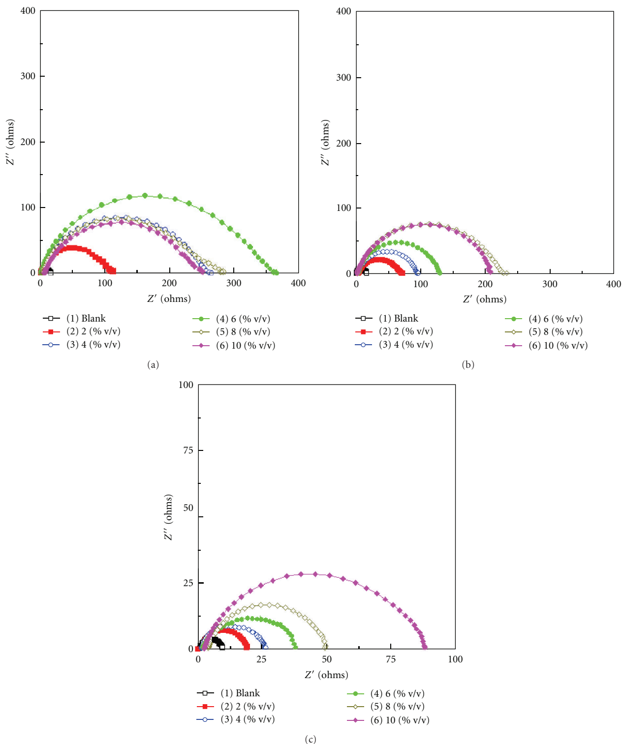
FIGURE 2: Impedance diagrams for mild steel in 1N HCl solution in the absence and presence of various concentrations of the plant extract (a) Ocimum sanctum , (b) Aegle marmelos , and (c) Solanum trilobatum .
