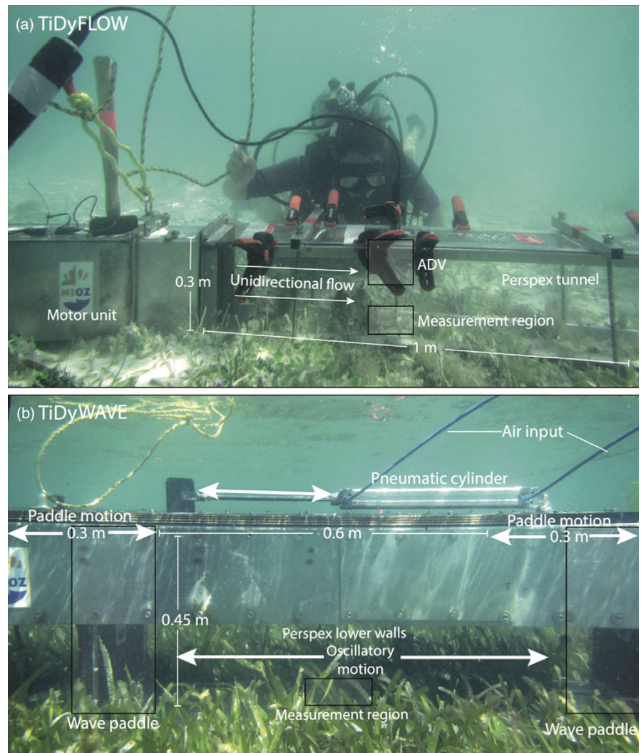
FIGURE 1 The TiDyFLOW flume (a) consists of a motor unit with two propellers that generate a unidirectional flow through the clear Perspex tunnel that is embedded into the sediment. The speed of the propellers is regulated to control the flow speed, with an ADV positioned in the centre of the tunnel, which records the flow velocity. Sediment movement is monitored beneath the ADV to determine the threshold flow velocity at which the sediment begins to move. The TiDyWAVE flume (b) mimics the oscillatory flow created by an unbreaking wave. Wooden wave paddles on either end of the flume move back and forth by the pneumatic cylinder observed on the top of the flume. The speed of the movement is controlled by regulating the airflow into the pneumatic cylinder. The time at which the boards moved back and forth in one cycle was calculated to be the oscillatory velocity. Clear Perspex surrounds the base of the flume allowing for the sediment movement within the flume to be observed [Colour figure can be viewed at wileyonlinelibrary.com ]
