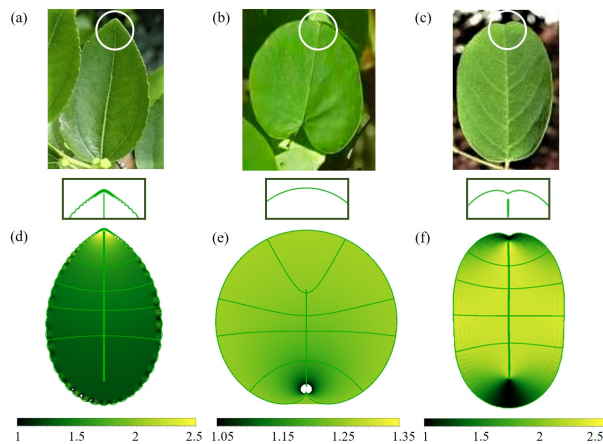
FIG. 2. Natural leaves: (a) Jujube leaf with sharp tip and oscillatory border. (b) Redbud leaf with rounded tip and smooth border. (c) Robinia pseudoacacia leaf with concave tip and smooth border. Mathematical images: (d)-(f) simulated by shape function (see SM, Sec. SII). Level of green colors shows the local growth density in different regions, lighter color indicating more growth intensity. Jujube leaf (a) and (d) grows more at the tip while the top and bottom of Robinia pseudoacacia leaf (c) and (f) have a weak level of growth. Redbud leaf (b) and (e) shows a relatively uniform growth in the entire area, except near the petiole.
