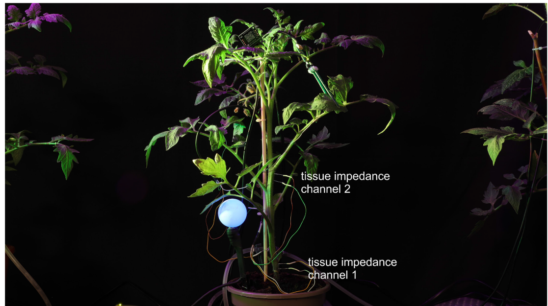
Figure 2. Setup with tissue impedance measurements (two independent channels) with tomato plants Solanum lycopersicum .
