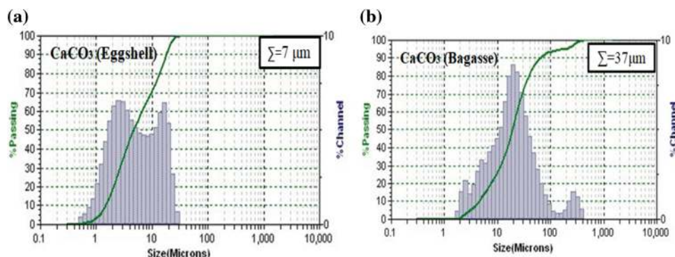
Figure 3: Particle size analyzer MICROTRAC. (a) \text{CaCO}_3 –Eggshell after the milled. (b) \text{CaCO}_3 – Agave salmiana bagasse ash after the milled
