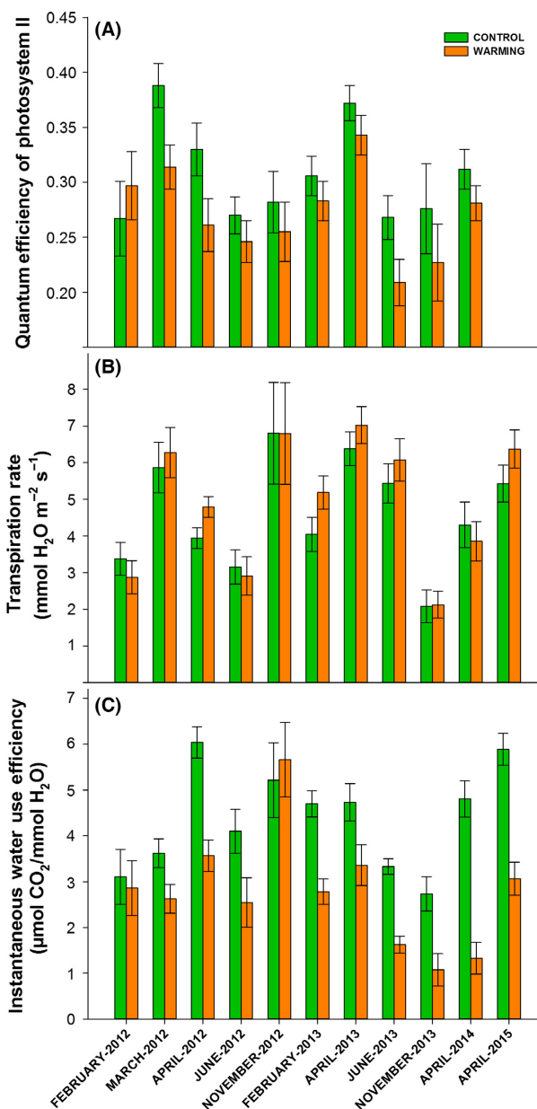
Figure 4. Quantum efficiency of photosystem II (A), transpiration rates (B), and instantaneous water-use efficiency values (C) in warmed and control plants at 10–11 different measurement dates spanning four consecutive growing seasons. Data represent means \pm SE ( n = 10 –15).
