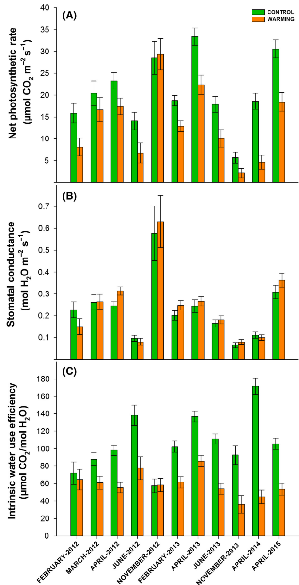
Figure 2. Mean net photosynthetic rates (A), stomatal conductance (B), and intrinsic water-use efficiency values (C) in warmed and control plants at 11 different measurement dates spanning four growing seasons. Data represent means \pm SE ( n = 10 –15).
