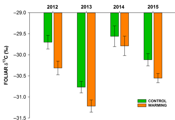
Figure 5. Mean leaf \delta^{13}\text{C} values in control and warmed plants at the peak of the growing season (April) in the 4 years of the study. Data represent means \pm SE ( n = 10\text{--}15 ).
