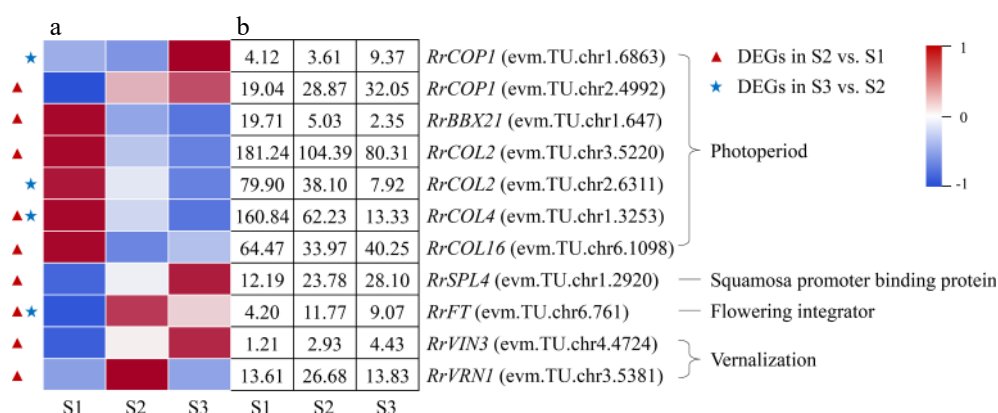
Fig. 8 Expression of photoperiod- and vernalization-related DEGs. (a) The expression heat map of DEGs. (b) The FPKM values of DEGs. BBX21: B-box 21; CO: CONSTANS; COL: CONSTANS-like; COP1: Constitutive Photomorphogenesis 1; FLC: Flowering Locus C; FT: Flowering locus T protein; SPL4: Squamosa promoter-binding-like protein 4; VIN3: Vernalization insensitive protein 3; VRN1: Vernalization protein 1
