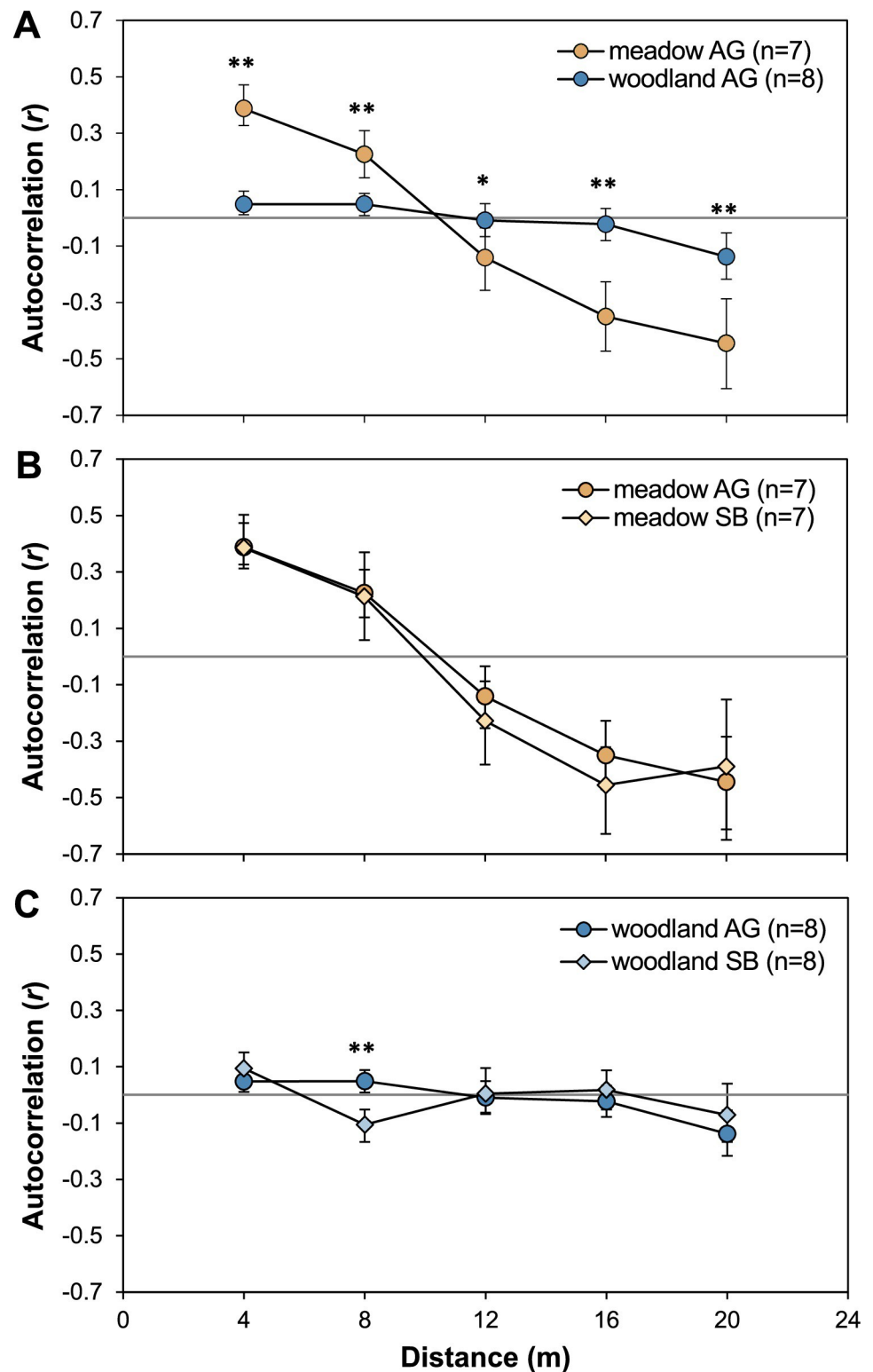
Fig 4. Correlograms of spatial genetic autocorrelation in populations of Viola elatior . Comparison of correlogram homogeneity is shown for (A) aboveground populations grouped for habitats, and for aboveground and seed bank populations from either only (B) meadow or (C) woodland habitats; \omega -test indicates overall significance (A: \omega = 73.74 , p = 0.0001 ; B: \omega = 9.33 , p = 0.497 ; C: \omega = 19.85 , p = 0.030 ). * p < 0.05 and ** p < 0.01 indicate significant differences for single distance classes. AG—aboveground; SB—seed bank.
