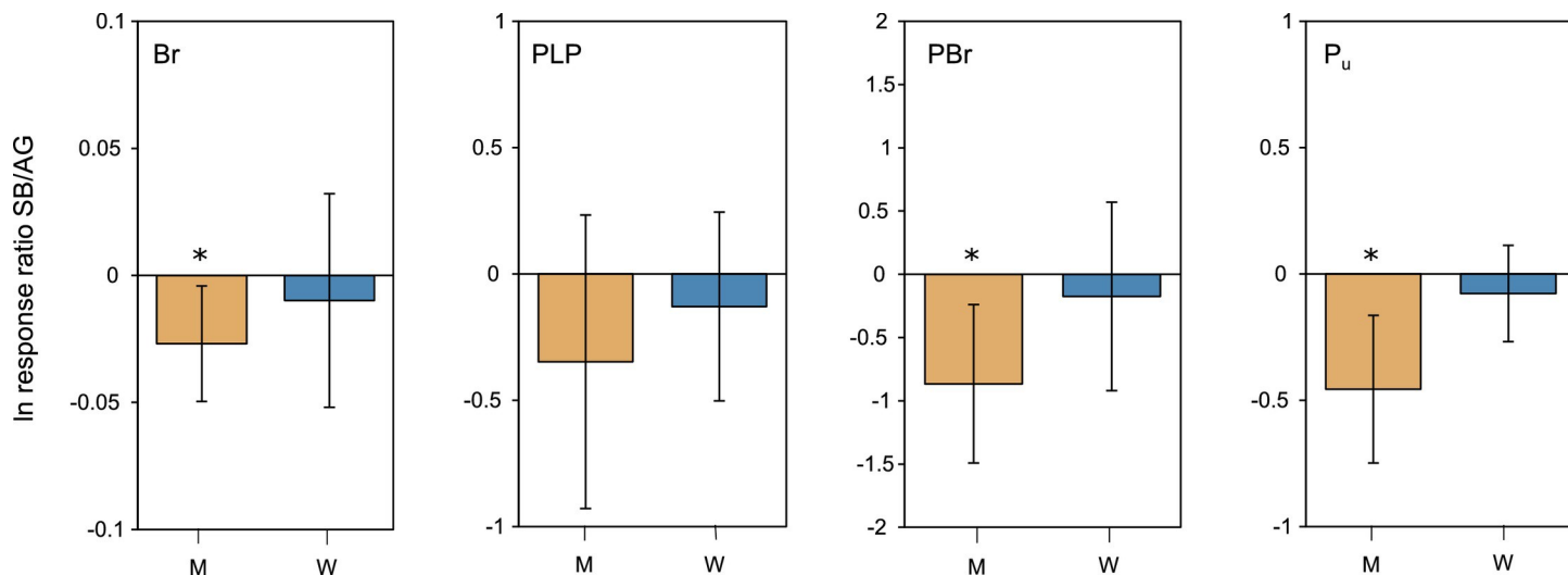
Fig 2. Mean ( \pm 95\% CI) ln response ratio of Br , PLP , PBr , and P u between seed bank and aboveground cohorts in meadow (M) and in woodland (W) habitats, respectively. Br —band richness, PLP —percentage of polymorphic loci at the 5% level; PBr —pairwise private band richness (aboveground vs. seed bank); P u —proportion of unique AFLP-phenotypes. Negative ln response ratios denote higher values in the aboveground cohort. Differences between aboveground and seed bank cohorts were considered significant when 95% CI did not overlap with zero.
