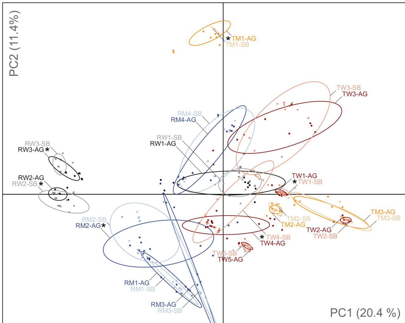
Fig 3. Principal component analysis (PCA) of the genetic structure in populations of Viola elatior . German populations are indicated by blue (meadow) and grey (woodland), and Czech populations by orange (meadow) and red (woodland). Aboveground and seed bank cohorts are depicted by strong and light colors, respectively. Inertia ellipses indicate dispersion of samples in relation to mean coordinates and include approximately three-fourths (76%) of all individuals for each group. Stars denote populations with significant genetic differentiation ( \Phi_{ST} ) between aboveground and seed bank cohorts (see also S3 Table ).
