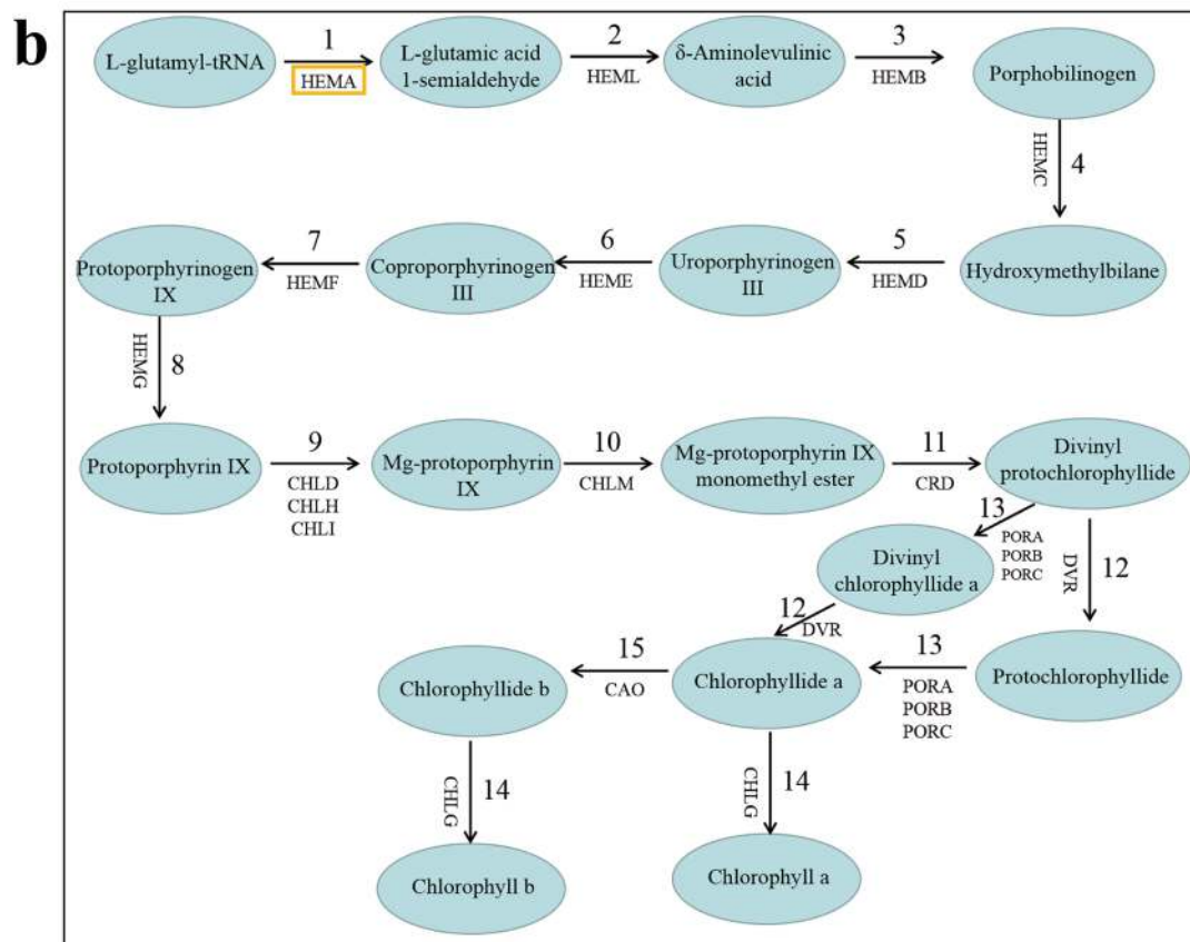
Figure 7. The down-regulated DEGs of “photosynthesis” pathway (a) and “chlorophyll biosynthesis” pathway (b).
