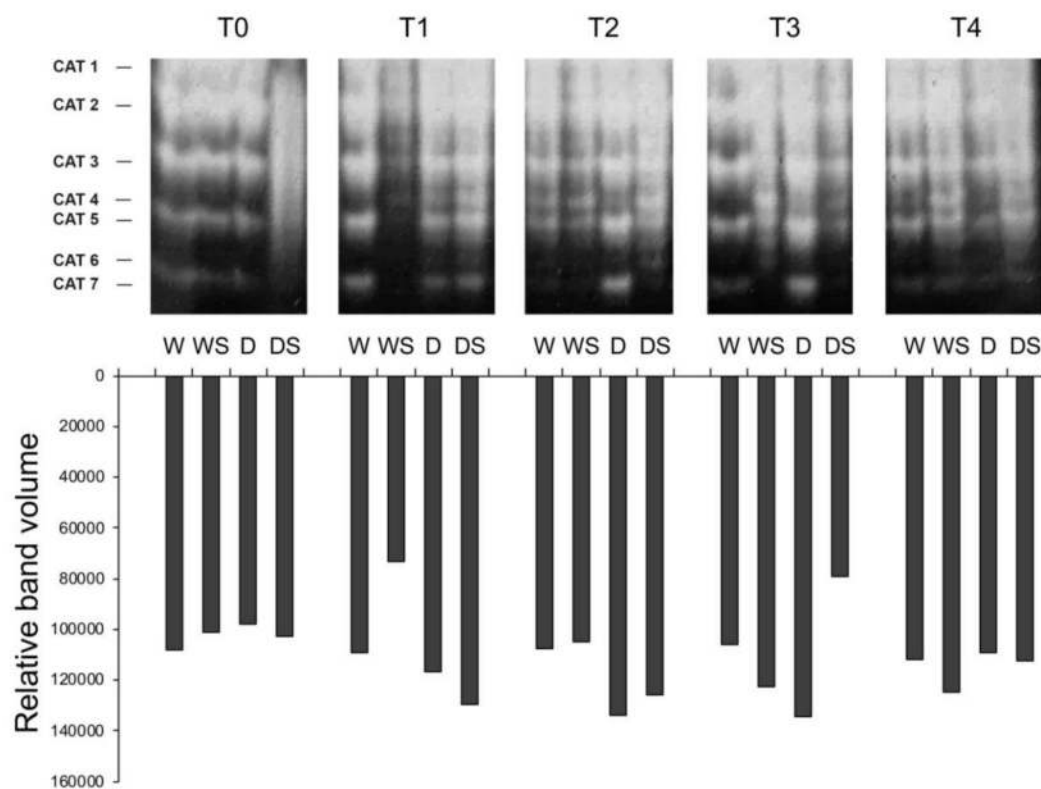
Figure 6. Zymograms of catalase (CAT) isoforms. Total soluble proteins isolated from leaves (35 µg protein/lane) of watered plants (W), drought-stressed plants (D), watered plants treated with SA (WS) or drought-stressed plants treated with SA (DS) were separated by native PAGE and assayed for CAT activity. T0–T4 are different sampling points (see Figure 1). Total CAT activities are represented by bars.
