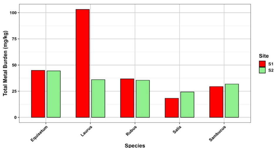
Fig. 5 Total metal burden in plant species at two sites (S1, S2)
