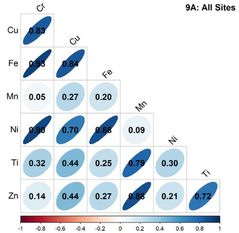
Fig. 9 Correlation matrices of metal concentrations: (A) all sites combined, (B) site S1, and (C) site S2
