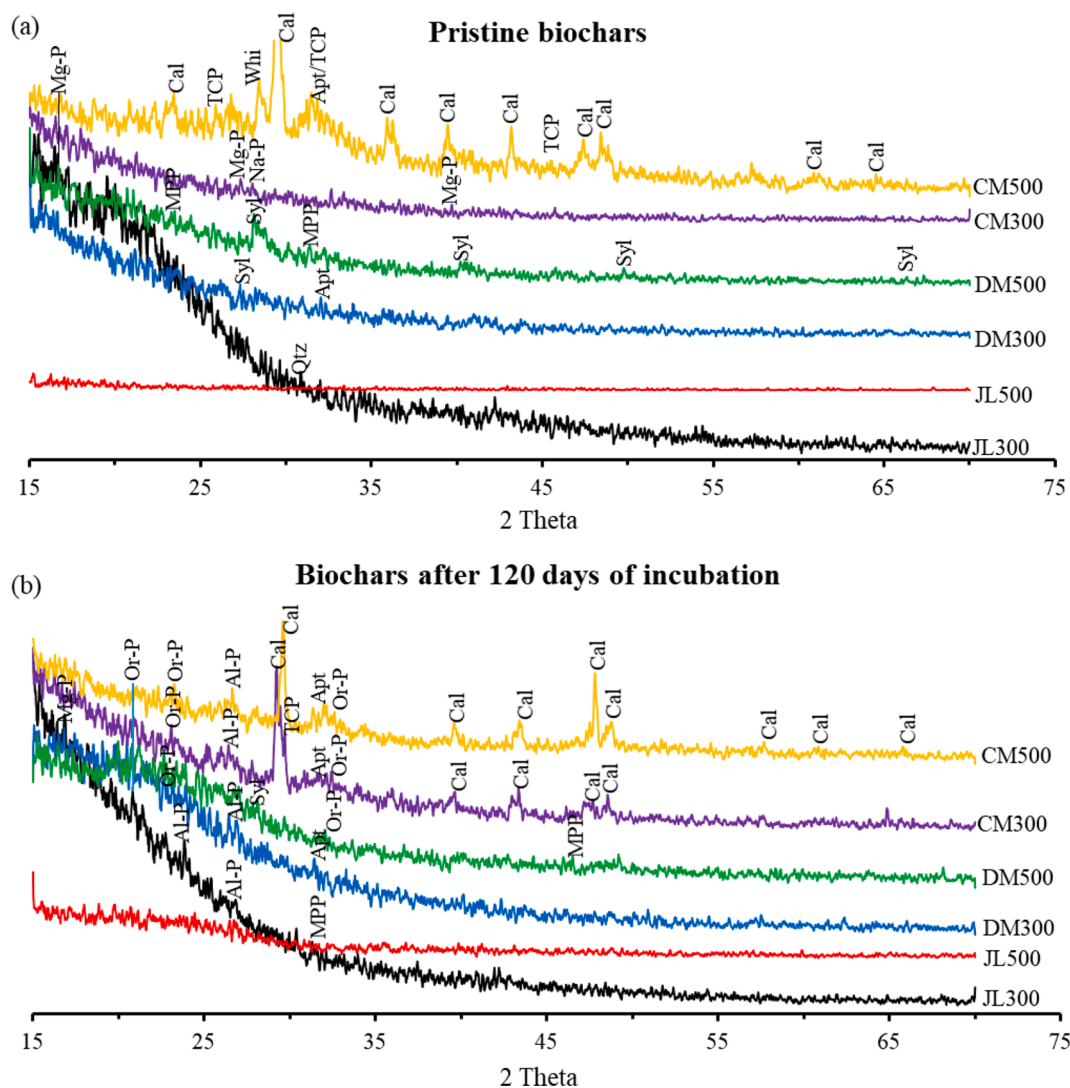
Fig. 6. XRD patterns of pristine biochars (a) and biochars after 120 days of incubation (b). Peaks of quartz (Qtz), calcite (Cal), sylvite (Syl), hydroxyapatite (Apt), monopotassium phosphate (MPP), magnesium phosphate hydrate (Mg-P), sodium dihydrogen phosphate (Na-P), tetracalcium phosphate (TCP), and whitlockite (Whi) minerals in XRD spectra are designated.
