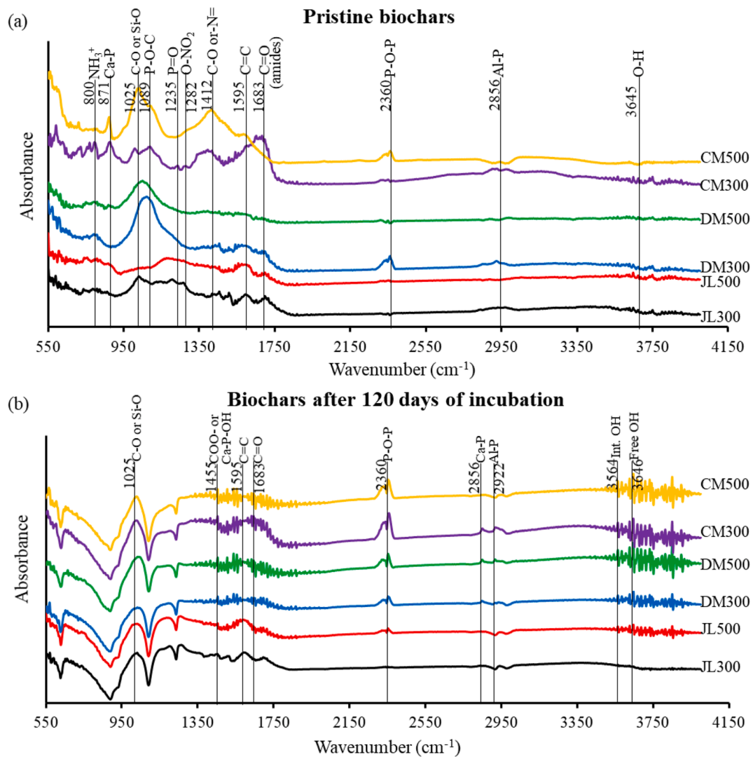
Fig. 5. FTIR-ATR spectra of pristine biochars (a), and biochars after 120 days of incubation (b). Major peaks of different functional groups are indicated.
