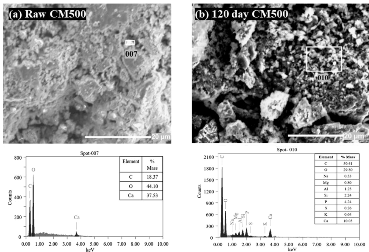
Fig. 7. Scanning electron micrographs (SEM) and associated energy dispersive X-ray spectroscopic (EDS) quantification of the CM500 biochar a) before and b) after 120 days of incubation.
