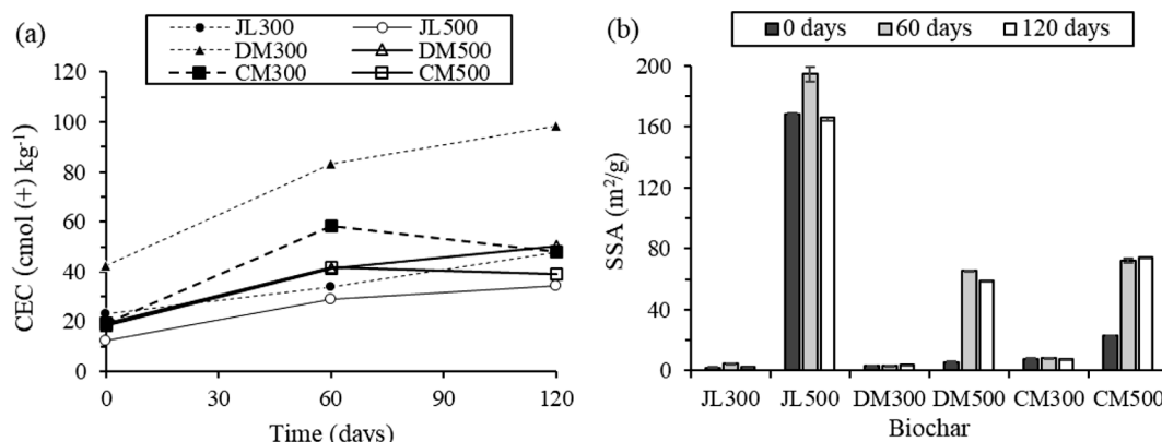
Fig. 8. Effect of incubation on biochar a) cation exchange capacity (CEC) and b) specific surface area (SSA).
