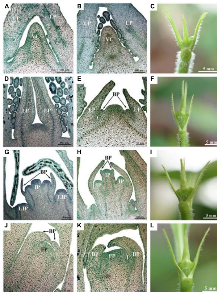
FIGURE 2 | Luculia gratissima morphological and histological characteristics, shoot apices at five time points upon short-day treatment. (A–C) Vegetative buds in the undifferentiated stage (SD0 to SD7). (D–F) Bract primordial differentiation stage (SD10). (G–I) Inflorescence primordial differentiation stage (SD13). (J–L) Floret primordial differentiation stage (SD19). (A,B,D,G,H) Histological images obtained from paraffin-embedded sectioned samples (scale bar: 100 \mu m). (E,J,K) Histological images obtained from paraffin-embedded sectioned samples (scale bar: 50 \mu m). (C,F,I,L) The external morphology of shoot apices at different developmental stages (scale bar: 5 mm). BP, bract primordia; FP, floret primordia; IP, inflorescence primordia; LIP, lateral inflorescence primordium; LP, leaf primordia; and VC, vegetative cone.
