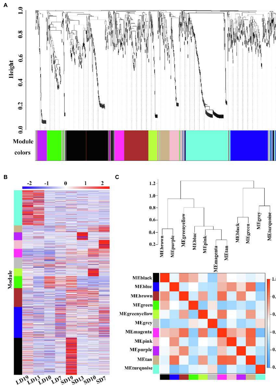
FIGURE 4 | Weighted co-expression network analysis of 1,226 DEGs at four developmental stages of L. gratissima , short- or long-day treatments. (A) Hierarchical cluster tree showing the co-expression modules, with each tree leaf representing one gene. The major tree branches constitute 11 modules labeled by different colors. (B) Heat map of gene relative expression of different modules (y-axis) in eight samples (x-axis). The Z-score normalized RPKM value for an individual gene at a given developmental stage is indicated in a green (low expression) to red (high expression) scale. (C) Eigengene network representing the relationships among the different modules. The hierarchical clustering dendrogram of the eigengenes shows the relationships among the modules, whereas the heat map shows the correlation between the different modules, with deeper red color representing a stronger correlation.
