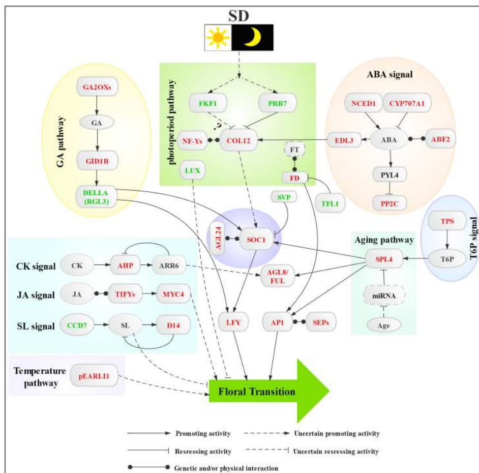
FIGURE 6 | Proposed regulatory network of short-day photoperiod-induced floral transition in L. gratissima . Colored fonts represent downregulated (green) or upregulated (red) genes.
