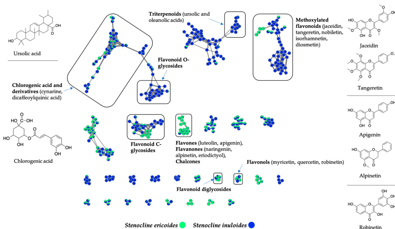
Figure 5. S. ericoides (green) and S. inuloides (blue) are polyphenol-rich species. The molecular networks were created by MetGem from the spectra file exported from Progenesis QI. The annotations correspond to standard or analogue matches to GNPS libraries and were performed using a similarity cosine scoring \geq 0.6 .
