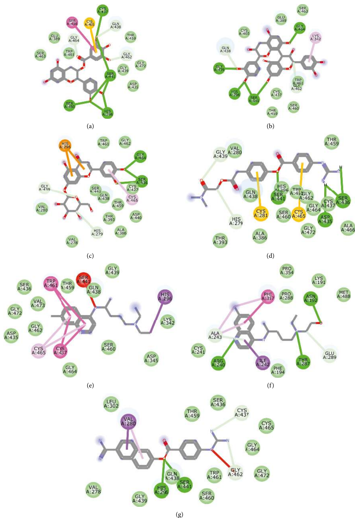
FIGURE 15: 2D representation of (a) 3-galloylcatechin, (b) proanthocyanidin B1, (c) luteolin 7-galactoside, (d) camostat, (e) chloroquine, (f) hydroxychloroquine, and (g) nafamostat in the binding pocket of TMPRSS2. Hydrogen, carbon-hydrogen, and \pi bonds are depicted as green, light blue, and any other coloured (purple, magenta, orange, turquoise blue, pink, and yellow) broken lines, while Van der Waal interactions appear as light green circles.
