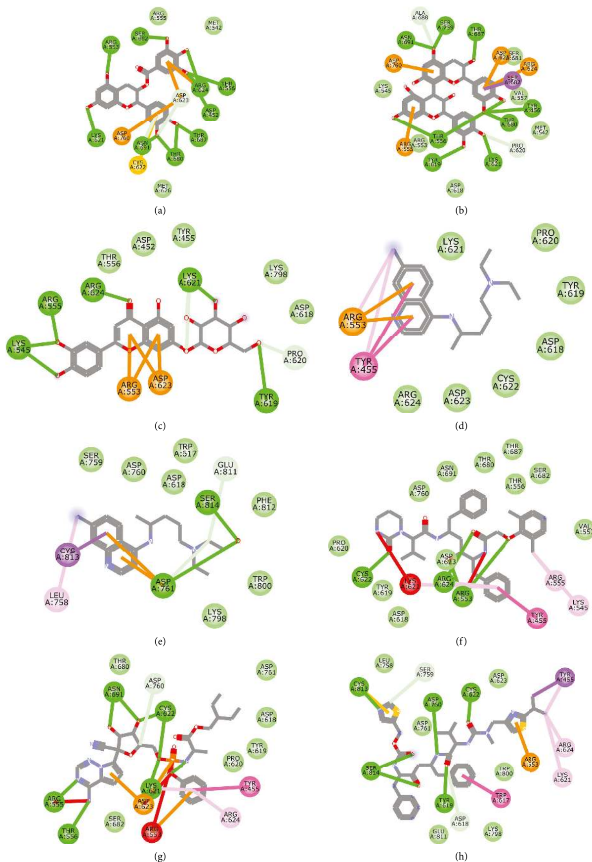
FIGURE 7: 2D representation of (a) 3-galloyl catechin, (b) proanthocyanidin B1, (c) luteolin 7-galactoside, (d) chloroquine, (e) hydroxychloroquine, (f) lopinavir, (g) remdesivir, and (h) ritonavir in the binding pocket of RdRp. Hydrogen, carbon-hydrogen, unfavourable, and \pi bonds are depicted as green, light blue, red, and any other coloured (purple, magenta, orange, turquoise blue, pink, and yellow) lines, while Van der Waal interactions appear as light green circles.
