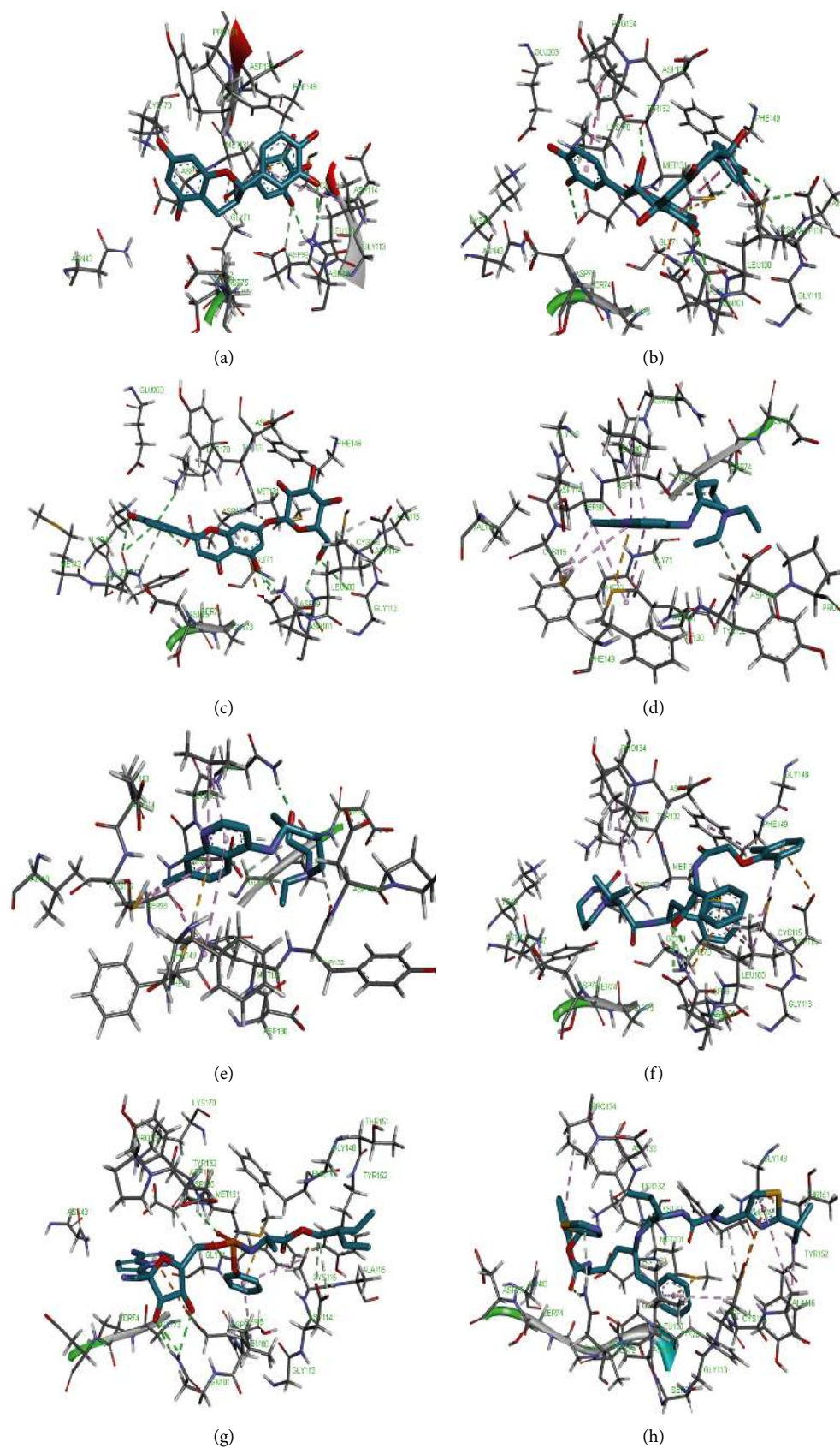
FIGURE 10: 3D representation of (a) 3-galloyl catechin, (b) proanthocyanidin B1, (c) luteolin 7-galactoside, (d) chloroquine, (e) hydroxychloroquine, (f) lopinavir, (g) remdesivir, and (h) ritonavir in the binding pocket of 2OMT.
