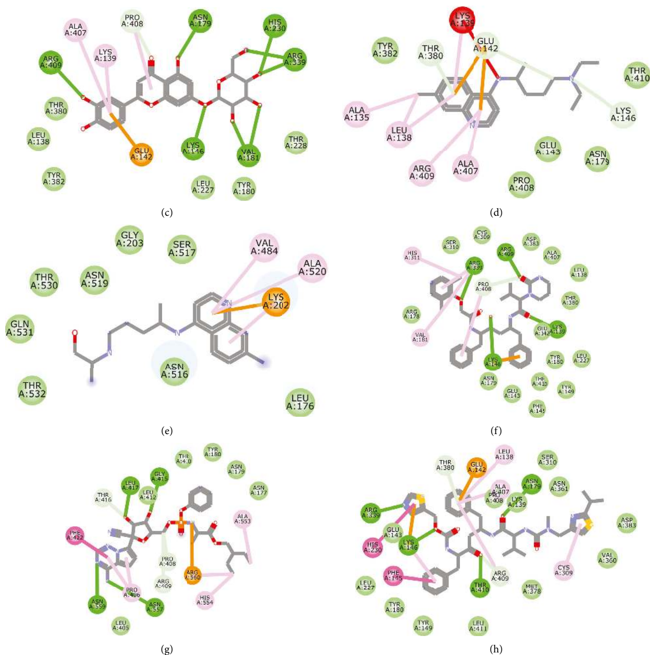
FIGURE 5: 2D representation of (a) 3-galloyl catechin, (b) proanthocyanidin B1, (c) luteolin 7-galactoside, (d) chloroquine, (e) hydroxychloroquine, (f) lopinavir, (g) remdesivir, and (h) ritonavir in the binding pocket of helicase. Hydrogen, carbon-hydrogen, and unfavourable and \pi bonds are depicted as green, light blue, red, and any other coloured (purple, magenta, orange, turquoise blue, pink, and yellow) lines, while Van der Waal interactions appear as light green circles.
