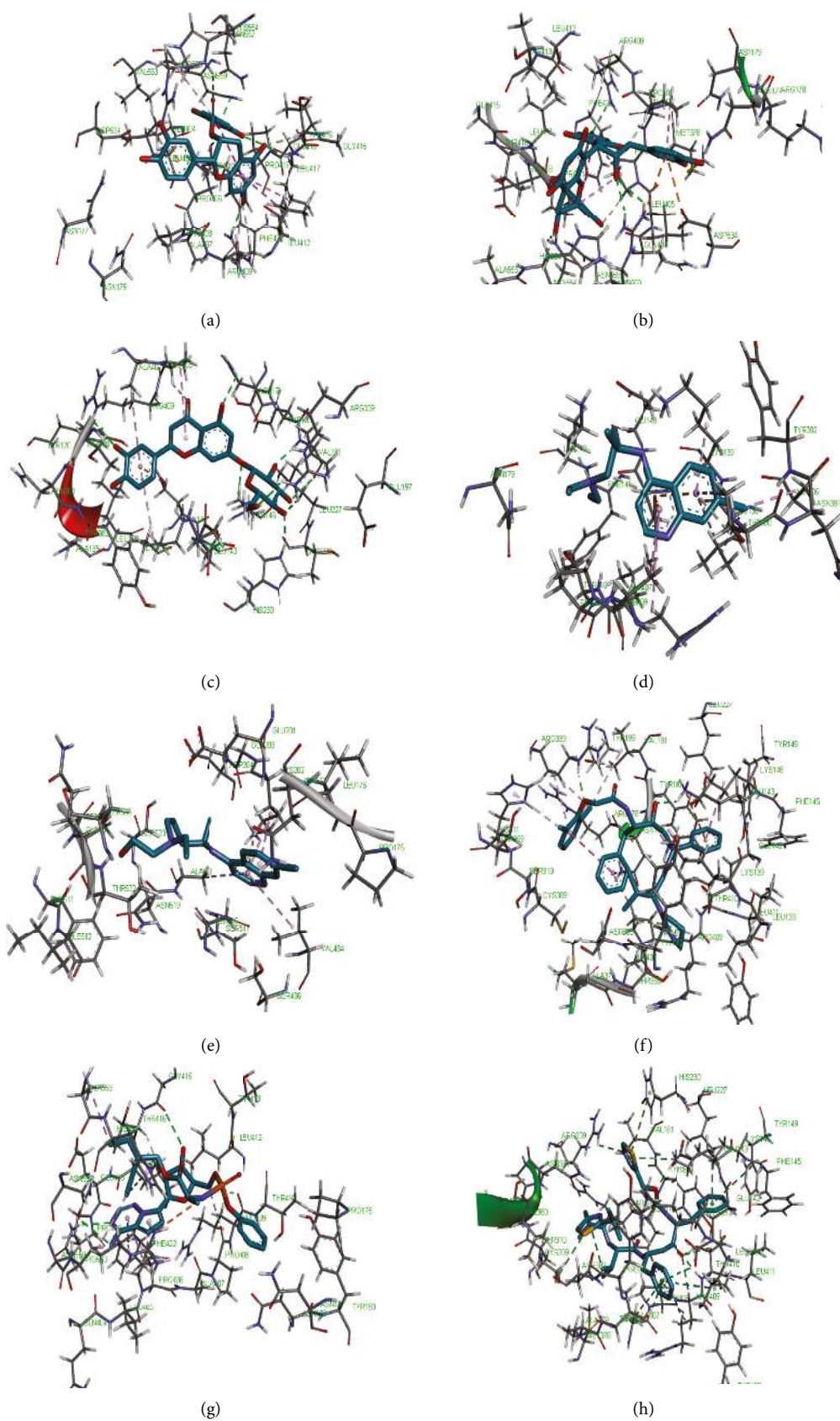
FIGURE 6: 3D representation of (a) 3-galloyl catechin, (b) proanthocyanidin B1, (c) luteolin 7-galactoside, (d) chloroquine, (e) hydroxychloroquine, (f) lopinavir, (g) remdesivir, and (h) ritonavir in the binding pocket of helicase.
