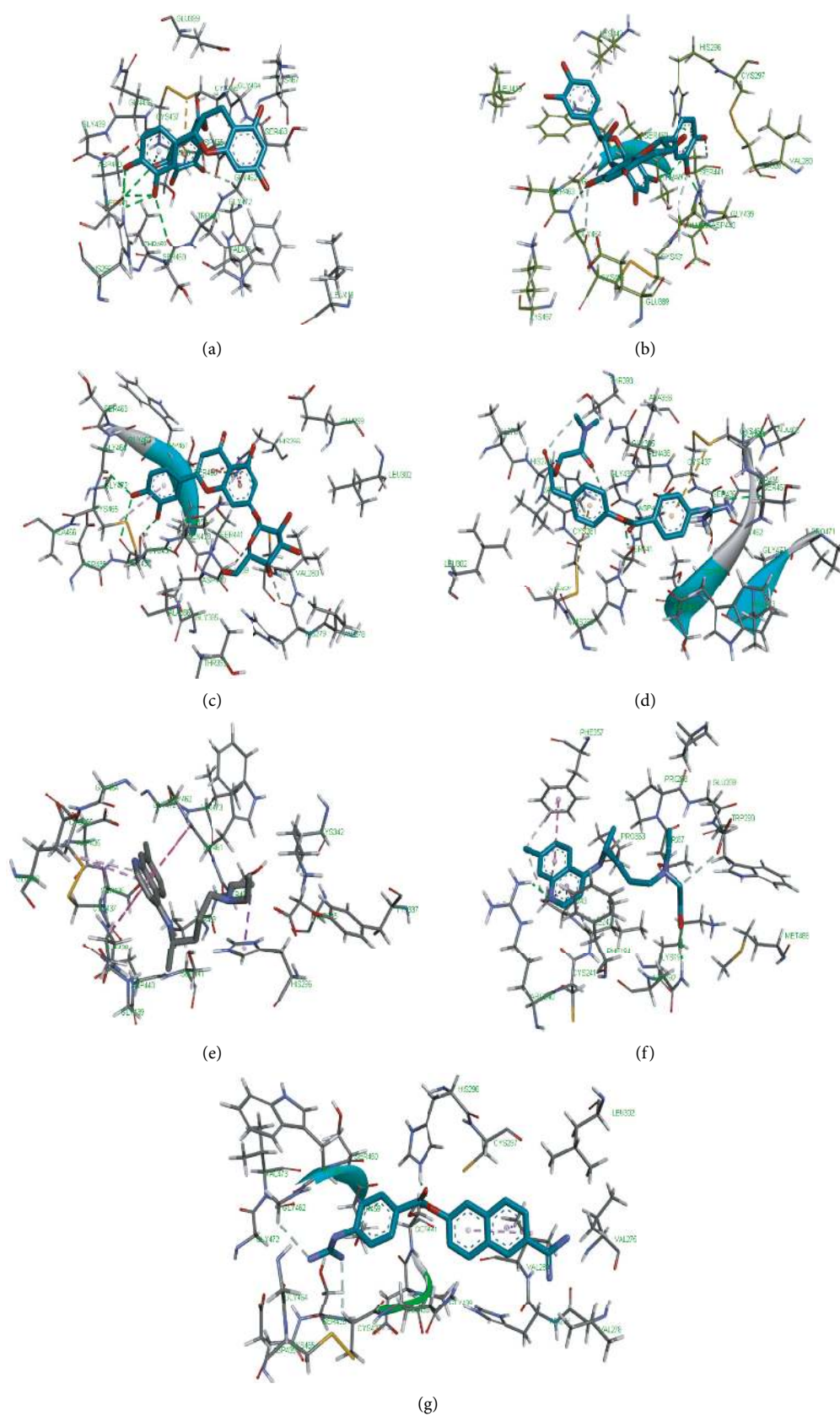
FIGURE 16: 3D representation of (a) 3-galloyl catechin, (b) proanthocyanidin B1, (c) luteolin 7-galactoside, (d) camostat, (e) chloroquine, (f) hydroxychloroquine, and (g) nafamostat in the binding pocket of TMPRSS2.
