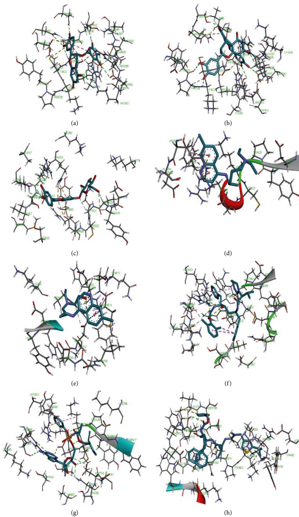
FIGURE 8: 3D representation of (a) 3-galloyl catechin, (b) proanthocyanidin B1, (c) luteolin 7-galactoside, (d) chloroquine, (e) hydroxychloroquine, (f) lopinavir, (g) remdesivir, and (h) ritonavir in the binding pocket of RdRp.
