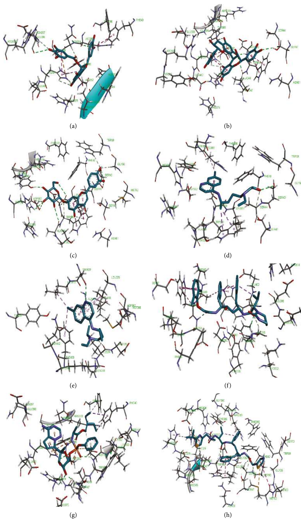
FIGURE 14: 3D representation of (a) 3-galloyl catechin, (b) proanthocyanidin B1, (c) luteolin 7-galactoside, (d) chloroquine, (e) hydroxychloroquine, (f) lopinavir, (g) remdesivir, and (h) ritonavir in the binding pocket of ACE2.
