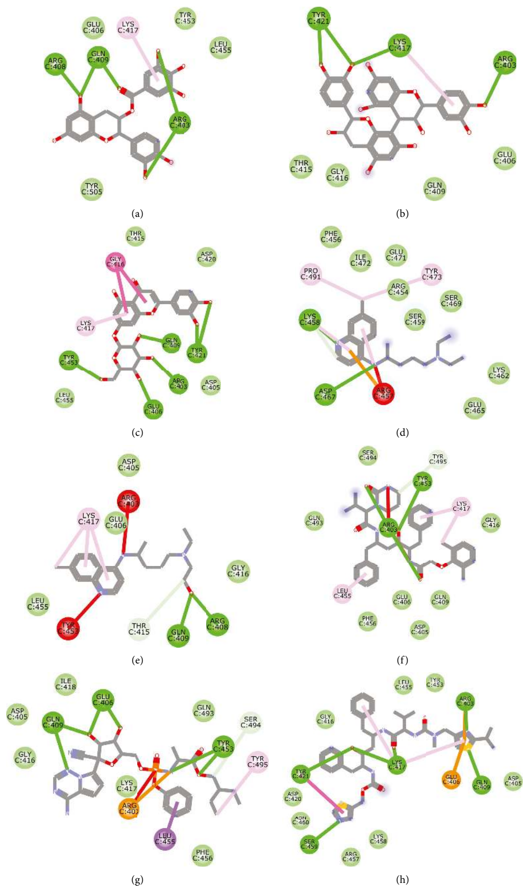
FIGURE 11: 2D representation of (a) 3-galloylcatechin, (b) proanthocyanidin B1, (c) luteolin 7-galactoside, (d) chloroquine, (e) hydroxy-chloroquine, (f) lopinavir, (g) remdesivir, and (h) ritonavir in the binding pocket of S-RBD. Hydrogen, unfavourable, and \pi bonds are depicted as green, red, and any other coloured (purple, magenta, orange, and pink) lines, while Van der Waal interactions appear as light green circles.
