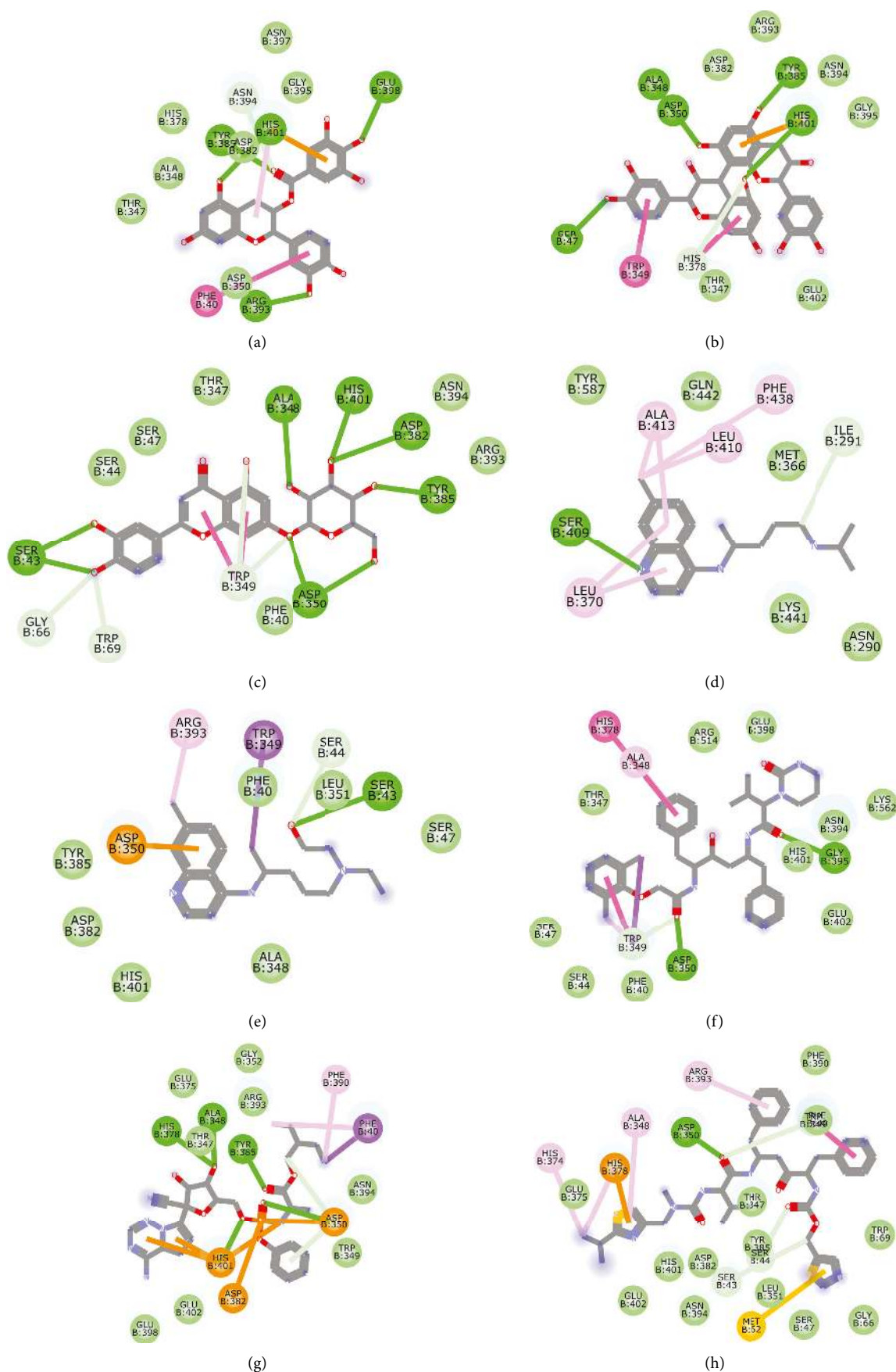
FIGURE 13: 2D representation of (a) 3-galloyl catechin, (b) proanthocyanidin B1, (c) luteolin 7-galactoside, (d) chloroquine, (e) hydroxy-chloroquine, (f) lopinavir, (g) remdesivir, and (h) ritonavir in the binding pocket of ACE2. Hydrogen and \pi bonds are depicted as green and any other coloured (purple, magenta, orange, turquoise blue, pink, and yellow) lines, while Van der Waal interactions appear as light green circles.
