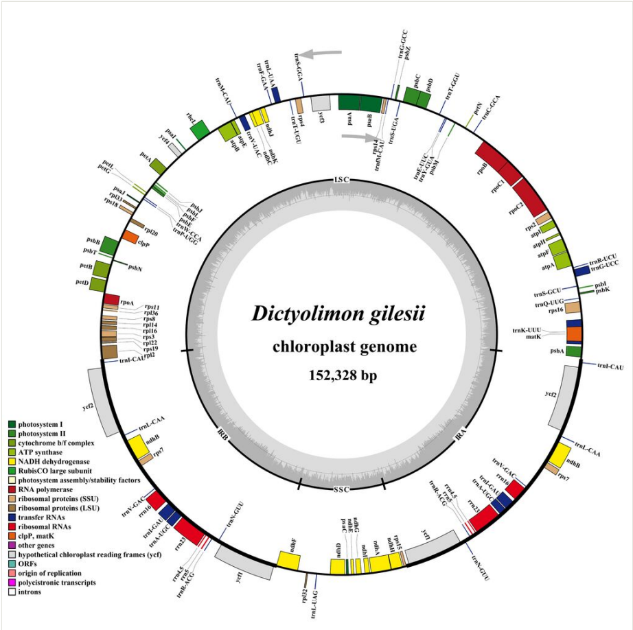
Figure 2. doi Circular genome map of the chloroplast genome of Dictyolimon gilesii . Genes shown on the inside of the circle are transcribed clockwise, genes on the outside are transcribed counterclockwise.
