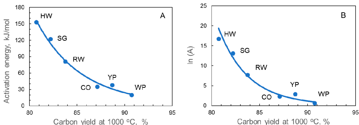
Figure 8. Relationship between kinetic parameters for oxidation by \text{CO}_2 at 800 °C and the carbon yield after isothermal pyrolysis in nitrogen at 1000 °C. The trend lines represent just a visual helper, with no implied significance.
