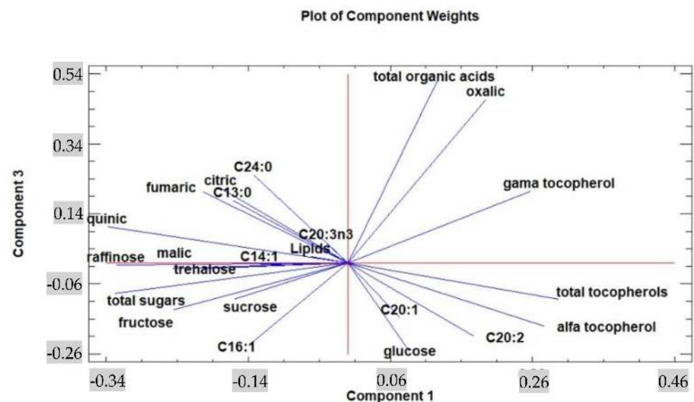
Figure 5. The loading plot of principal components 1 and 3 for the tested variables at different maturation stages of cardoon blades.
