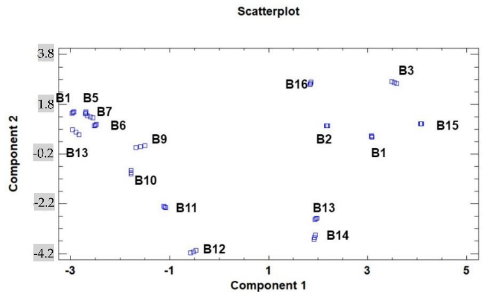
Figure 2. Two-dimensional scatterplot of principal components 1 and 2 for the tested variables at different maturation stages of cardoon blades (samples B1–B16).
