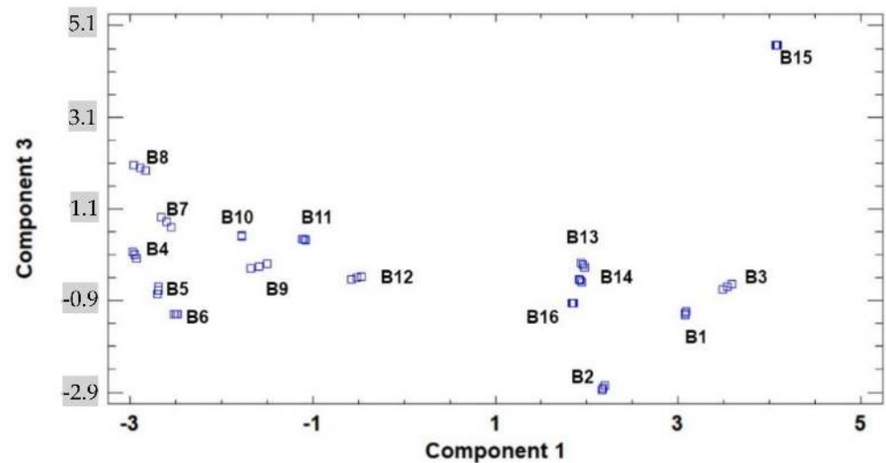
Figure 4. Two-dimensional scatterplot of principal components 1 and 3 for the tested variables at different maturation stages of cardoon blades (samples B1–B16).
