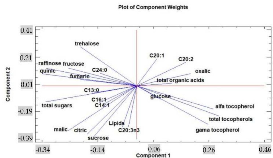
Figure 3. The loading plot of principal components 1 and 2 for the tested variables at different maturation stages of cardoon blades.
