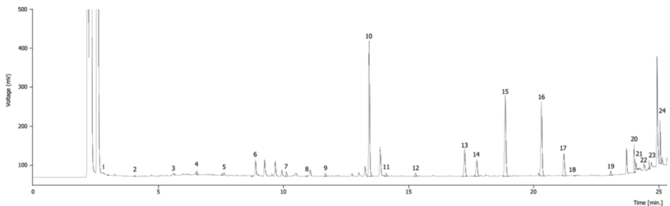
Figure 1. Fatty acids chromatogram of Cynara cardunculus L. var. altilis blades (sample B4, PGS 2). 1. C6:0—caproic acid; 2. C8:0—caprylic acid; 3. C10:0—capric acid; 4. C11:0—undecanoic acid; 5. C12:0—lauric acid; 6. C13:0—tridecanoic acid; 7. C14:0—myristic acid; 8. C14:1—tetradecanoic acid; 9. C15:0—pentadecanoic acid; 10. C16:0—palmitic acid; 11. C16:1—palmitoleic acid; 12. C17:0—heptadecanoic acid; 13. C18:0—stearic acid; 14. C18:1n9c—oleic acid; 15. C18:2n6c—linoleic acid; 16. C18:3n3—linolenic acid; 17. C20:0—arachidic acid; 18. C20:1—gadoleic acid; 19. C21:0—heneicosanoic acid; 20. C22:0—behenic acid; 21. C22:1—eicosenoic acid; 22. C20:5n3—eicosapentaenoic acid; 23. C23:0—tricosanoic acid; 24. C24:0—lignoceric acid.
