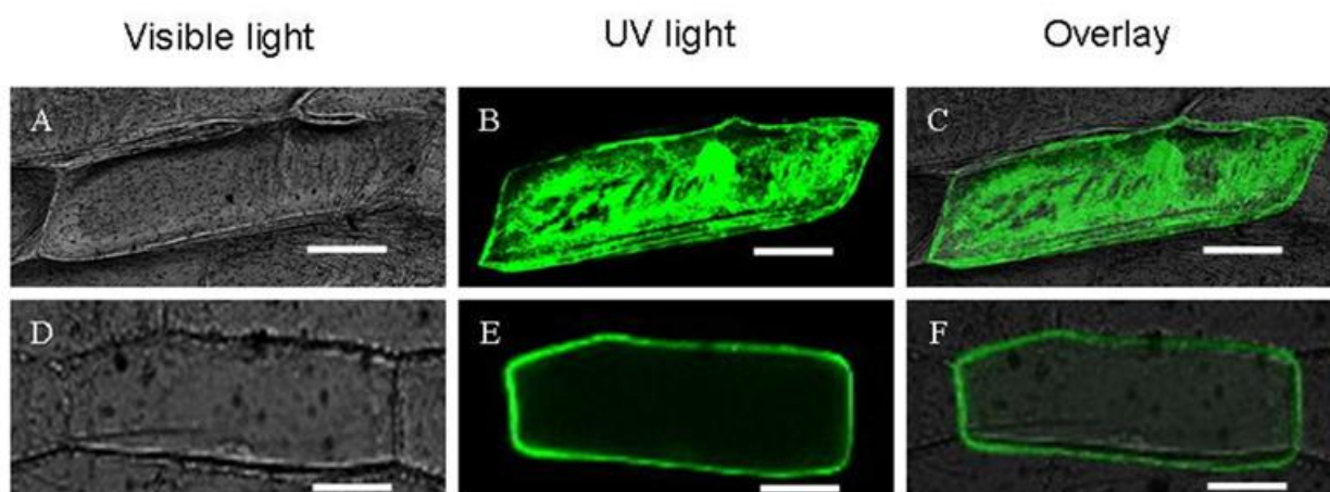
Figure 8. Subcellular localization of CaMV 35S::GFP and CaMV35S:: psoRPM1 -eGFP fusion constructs in onion epidermal cells by transient expression. The photographs were taken in the bright light filed for the morphology of the cell (A and D), in dark field for green fluorescence (B and E) and overlay images (C and F), respectively, for p35S::eGFP control plasmid (A-C) and p35S:: psoRPM1 -GFP plasmid (D-F). The scale bar indicates 100 \mu m.
