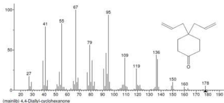
Fig 3.4: 4,4-Diallyl-cyclohexanone
