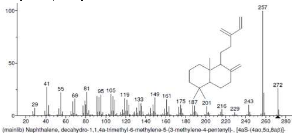
Fig. 4.1.3: Naphthalene
