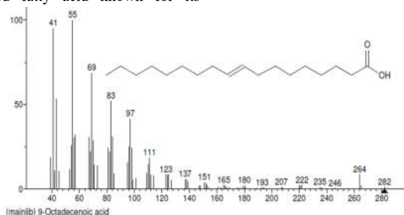
Fig 3.2.5: 9-Octadecenoic Acid
