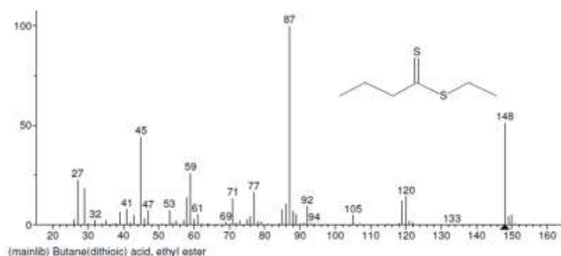
3.6.1: Butane(dithioic) Acid
