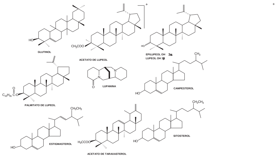
Figure 1. Some compounds isolated from Vernonthura patens .
