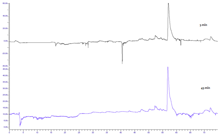
Figure 7. HPLC chromatographic profile of the ethanolic extract of the flowers of Vernonia patens obtained with 5 and 45 min of ultrasound extraction
