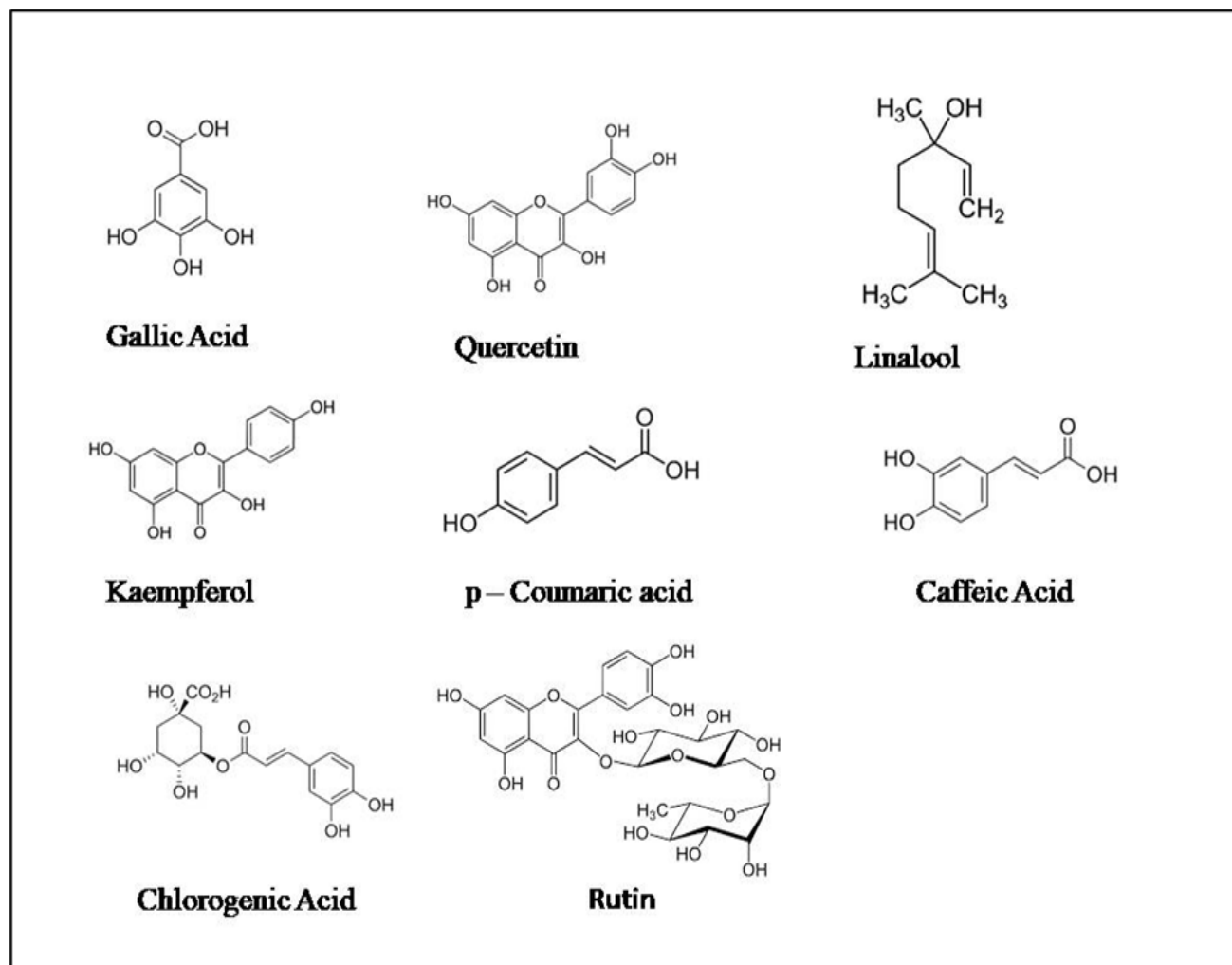
Fig. 2: Chemical Constituents of Jasminum sambac
