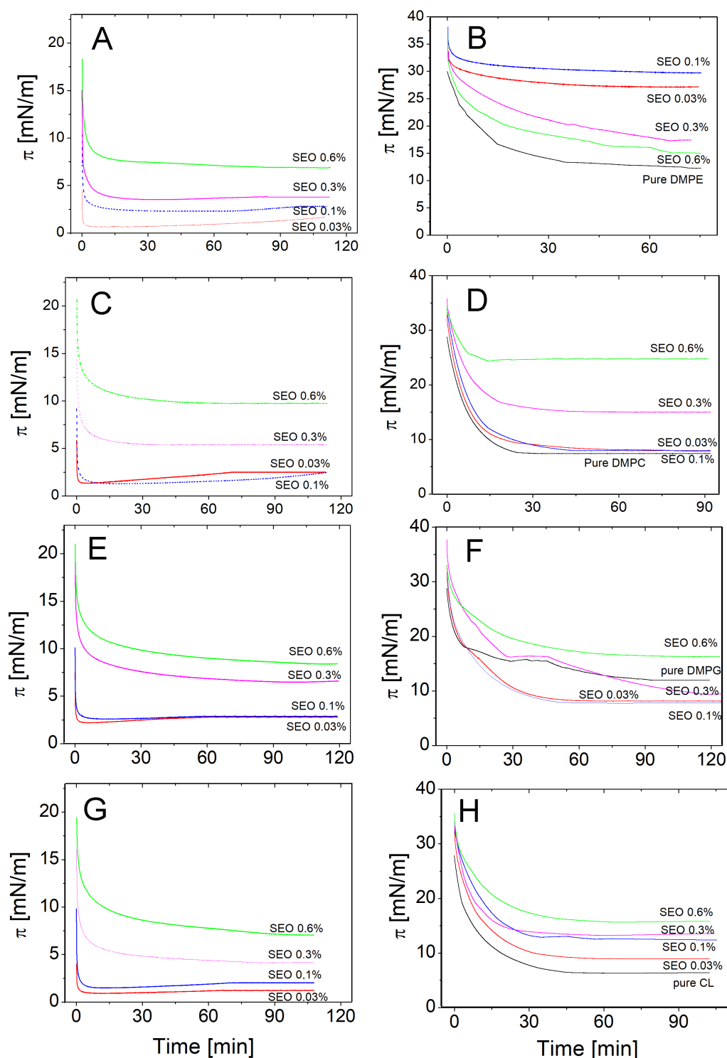
Figure A2. Relaxation behaviour of lipid monolayers after SEO injection at null surface pressure ( left panels ) and at 30 mN/m ( right panels ) for DMPE ( A,B ), DMPC ( C,D ), DMPG ( E,F ), and CL ( G,H ). Note the non-monotonous relaxation behaviour of DMPG upon injection of SEO at 30 mN/m (panel F ), in the surface pressure range of 10–20 mN/m, where the LE-LC transition occurs.
