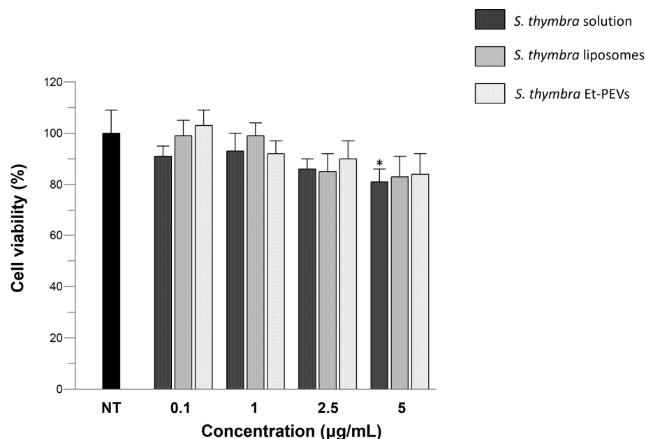
Figure 5. Effects of the S. thymbra ethanol solution and S. thymbra liposomes/Et-PEVs on the viability of HaCaT cells incubated for 24 h with different concentrations (0.1–5 \mu\text{g} /mL). *: p < 0.05 vs. non-treated control cells (NT).
