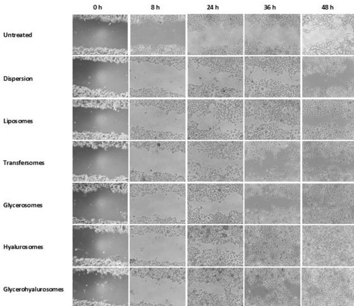
Figure 6. Representative images of the scratch performed in fibroblast monolayers and treated with the extract in dispersion or loaded in vesicles.
