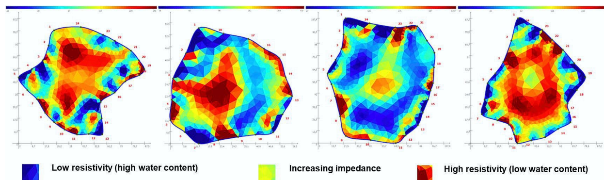
Figure 6: Individuals with low electrical conductivity regions with a previously identified presence of cavities based on Electrical Resistance Tomography (ERT).
