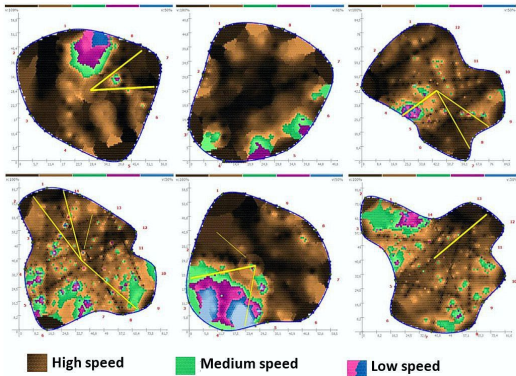
Figure 3: Measurements of sections of Spathodea campanulata individuals exhibiting internal trunk defects in lesser proportions as determined by sonic tomography (SoT).
