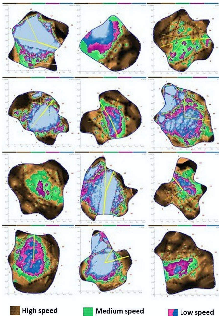
Figure 2: Measurements of the trunk sections of Spathodea campanulata individuals exhibiting prominent internal condition defects using sonic tomography (SoT).
