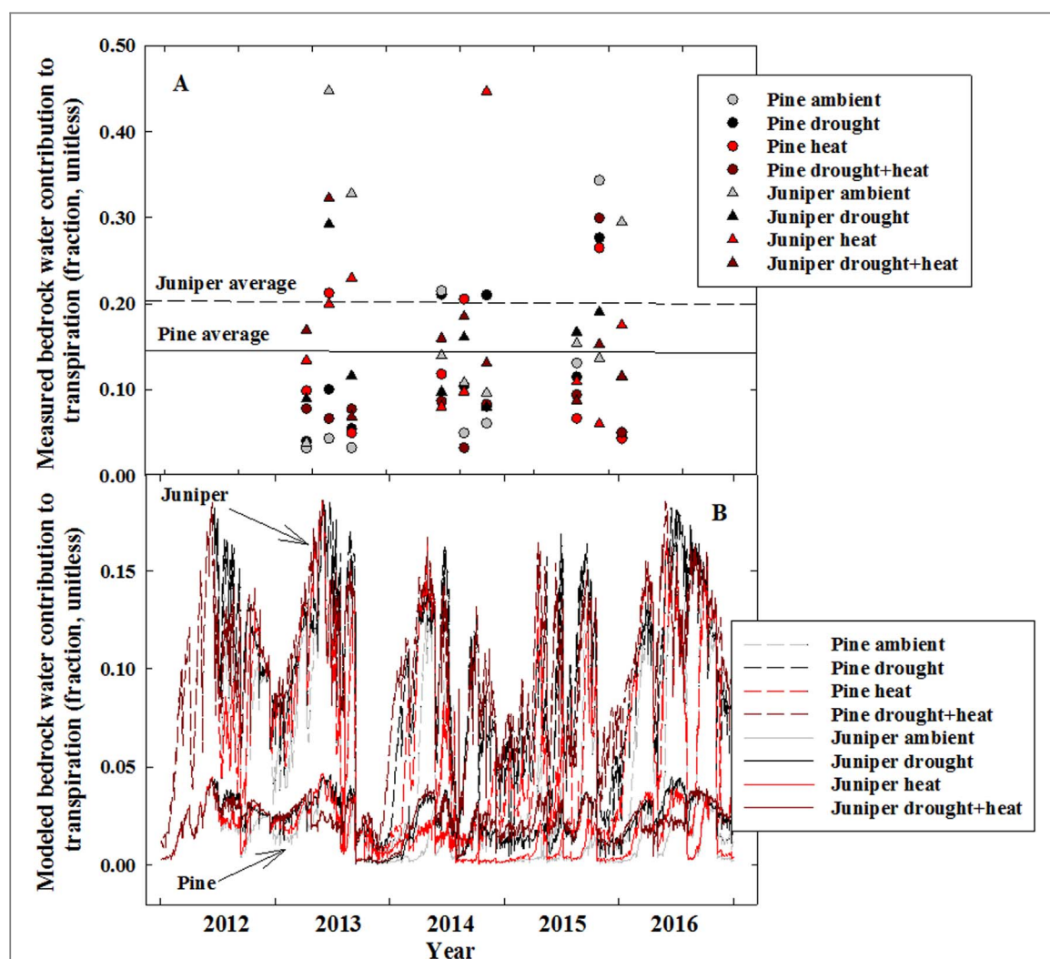
Figure 4. Deep water is a mechanism of persistence under drought and heat. (A) Deep water contribution to xylem water using natural abundance water isotope sampling for 2013–2015, and (B) TREES simulations of deep water contribution to transpiration. Both (A) and (B) suggest both species had persistent access to deep water. The depth to bedrock in this ecosystem is ~40–80 cm. (A) Re-calculated from Grossiord et al (2017a). See Grossiord et al (2017a) for detailed analyses of treatment impacts on bedrock water use.
