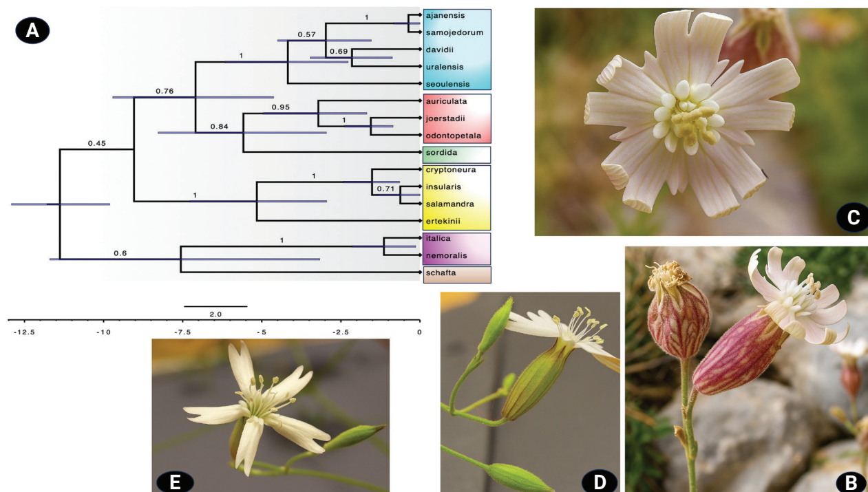
Figure 1. A. Maximum clade credibility species tree estimated from alignments of four nuclear and one chloroplast (cpDNA) region across 16 Silene species under a strict molecular clock. This model was preferred according to a model selection procedure based on marginal likelihood estimates of competing models. Phylogenetic analysis was conducted using the multispecies coalescent model in StarBEAST3. Branches are annotated with posterior probabilities, and blue bars at nodes indicate 95% highest posterior density (HPD) intervals for node heights, reflecting uncertainty in divergence times. Tip labels are coloured by sectional assignment within Silene . The scale bar represents substitutions per site, and the time axis (in Ma, million years ago) shows estimated divergence times, including the split between S. subg. Behenantha and S. subg. Silene and their respective lineages. Photographs show (B, C) calyx and petal morphology of S. odontopetala and (D, E) calyx and petal morphology of S. sordida grown under greenhouse conditions. Photo credits: (B, C) Kemal Yıldız; (D, E) Zeynep Toprak. Figures were generated using FigTree v1.4.4 and Inkscape v1.1.1.
