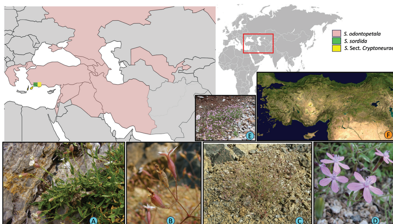
Figure 3. Map illustrating the approximate known geographic distributions of Silene sordida (green), S. odontopetala (rose), and sect. Cryptoneurae (yellow). Distribution data were compiled from GBIF (gbif.org), “Flora of Turkey and the East Aegean Islands” (Davis 1965–1985), and POWO (powo.science.kew.org) based on country-level records. Photographs: A. S. odontopetala (habit); B. S. sordida (flower); C. S. sordida (habit); D. S. ertekinii (flower); E. S. ertekinii (habit); F. geographical map of Anatolia. Photo credits: A–C. Kemal Yıldız; D–E. Zeynep Toprak. Figure generated using Python 3.13, Inkscape 1.1.1, and Microsoft PowerPoint 16.78.
