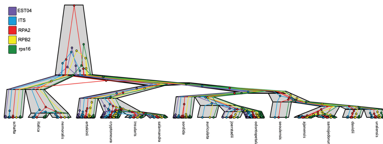
Figure 2. Schematic representation of the compatibility of the five gene trees with their species tree, obtained using UglyTrees (Douglas 2021). Coloured circles represent sampled sequences for 16 species and their inferred coalescent events traced backward in time, as estimated by StarBEAST3 under the multispecies coalescent model. Gray bars delineate species boundaries and the most recent common ancestors of those species. For visualization purposes, the widths of the species branches are not scaled to reflect the effective population sizes of the corresponding lineages.
