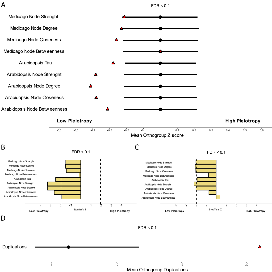
Fig. 4. Orthogroups with repeated sweeps tend to be less pleiotropic and harbour more duplications. (A) Pleiotropy assessment of the relaxed set of 107 orthogroups with FDR < 0.2, against 10,000 random draws. Red triangles represent the average pleiotropy of the candidate set, while black circles represent the mean of 10,000 random draws. Black lines represent the 95% interval of the random draws means. Each row represents a different pleiotropy measure, labelled on the left. (B) Pleiotropy Stouffer's Z of the top 33 orthogroups (FDR < 0.1), calculated using different pleiotropy measures labelled on the left. Dotted lines delimit the 95% confidence interval. (C) Pleiotropy Stouffer's Z for the more conservative set of 15 orthogroups identified by intersecting the 33 candidate OGs of the main analysis (FDR < 0.1) with results derived from nine additional PicMin omitting closely related Eucalyptus and Helianthus species. Dotted lines delimit the 95% confidence interval. (D) Duplication bootstrapping assessment of the top 33 orthogroups (FDR < 0.1) against 10,000 random draws. The red triangle represents the average duplication number in the candidate set of orthogroups, while the black circle and line represent mean and 95% interval of 10,000 random draws respectively.
