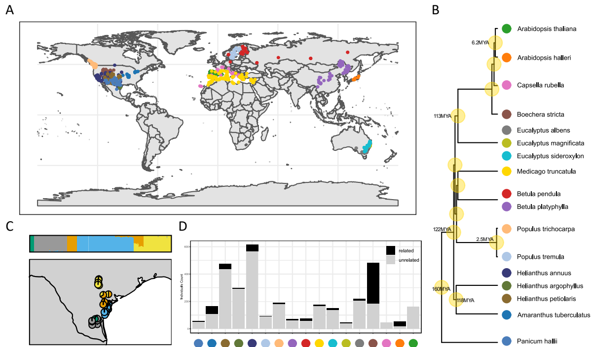
Fig. 1. Geographical distribution and relatedness within and among the study species. (A) Sampling locations of the 17 datasets included in the study. (B) Time-calibrated phylogenetic tree (retrieved from https://timetree.org/ ) of the 17 datasets, based on 12 reference species. (C) fastSTRUCTURE ancestry pie plot ( K = 5 ) of the Helianthus argophyllus dataset in Texas (USA), showing substantial sub structuring. (D) Relatedness filtering summary bar plot by dataset. Datasets labelled by corresponding colour from B.
