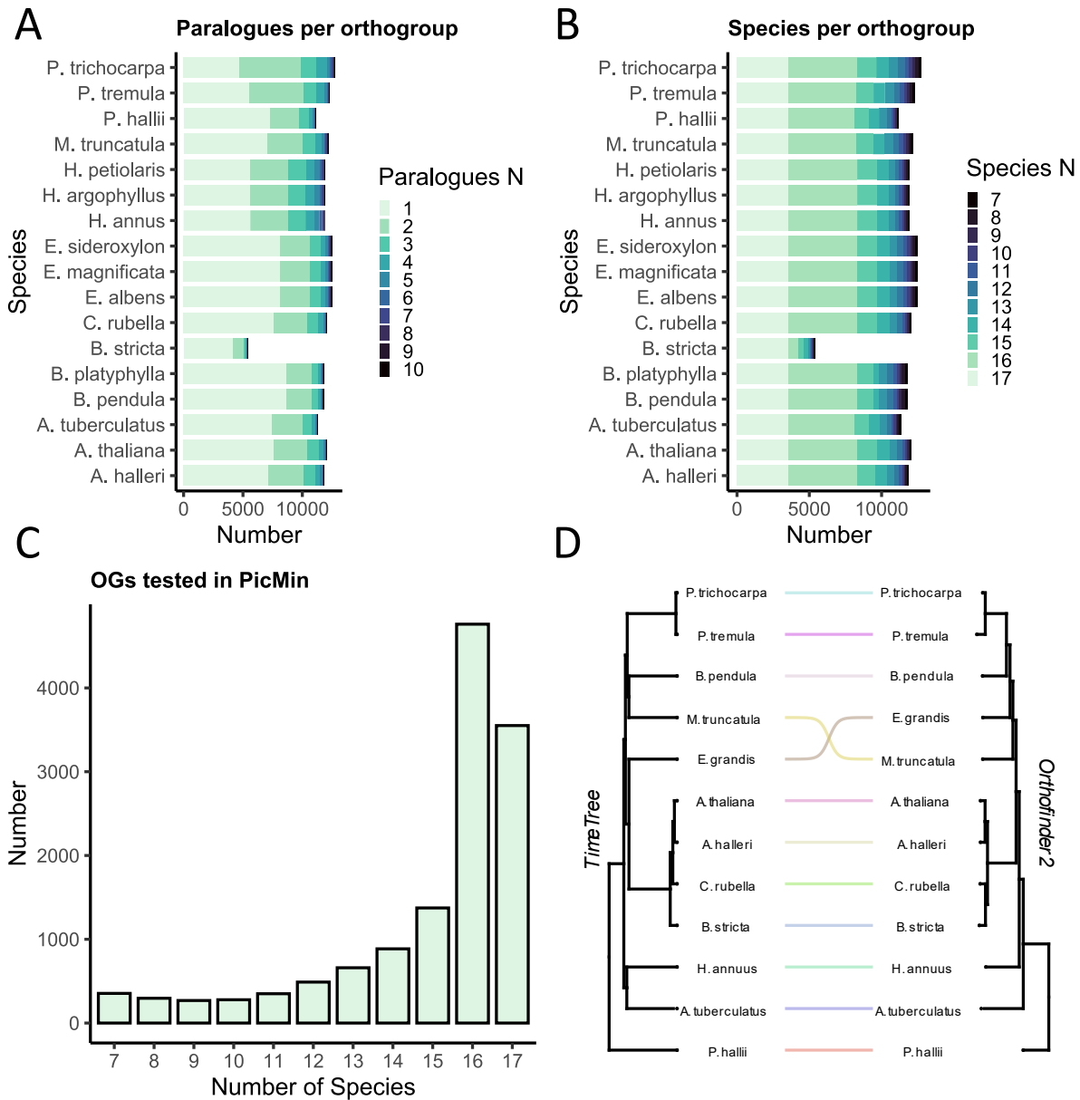
Fig. 2. Orthology assignment summary of the final set of 13,268 orthogroups. (A) Bar plot of the number of paralogues per orthogroup for each species. (B) Bar plot of the number of species included in each orthogroup, for the orthogroups of each species. (C) Distribution of the 13,268 tested orthogroups across species number. (D) Comparison between the TimeTree and Orthofinder2 phylogenies, each based on 12 reference species.
