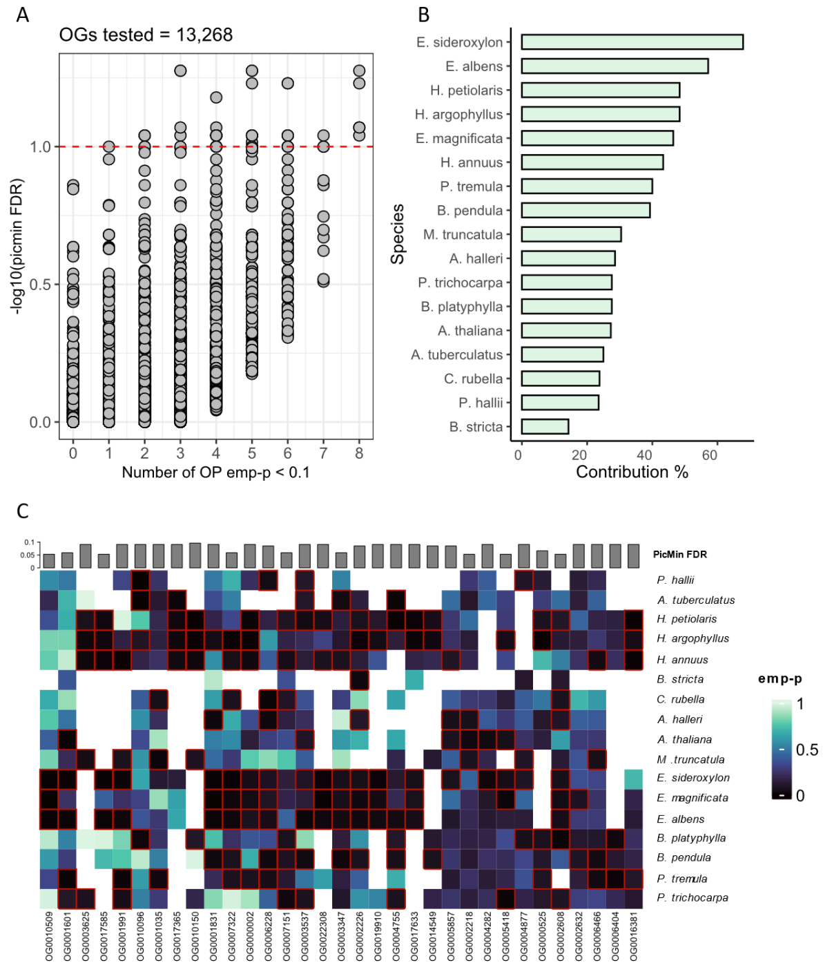
Fig. 3. Evidence for repeated selective sweeps across multiple species. (A) Distribution of PicMin FDR ( -\log_{10} PicMin FDR on the Y axis) for the 13,268 tested orthogroups, ordered by number of putative driving genes on the X axis (number of OmegaPlus emp-p < 0.1). Points above the red line have FDR < 0.1. (B) Species contribution to PicMin top candidates (FDR < 0.1), calculated for each species as: [number of empirical p-values < 0.1 in the PicMin FDR < 0.1 orthogroups]/[total number of orthogroups with PicMin FDR < 0.1 tested]. (C) Heatmap of OmegaPlus empirical p-values for the 33 candidate orthogroups ( PicMin FDR < 0.1); driving genes cells (emp-p < 0.1 – black cells) are outlined in red, species are ordered by phylogenetic distance along the Y axis. A white cell indicates that an orthogroup was not tested in a species.
