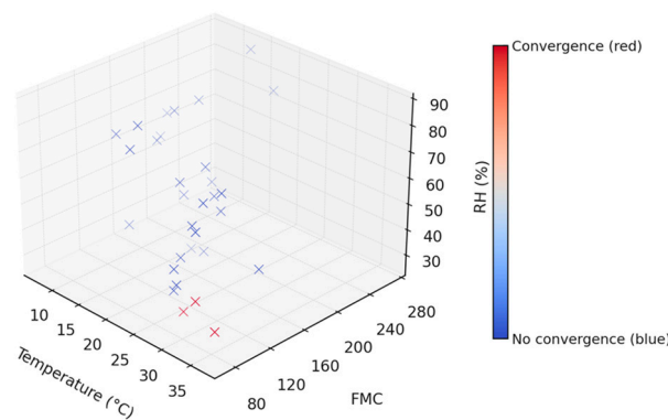
Figure 4. Three-dimensional representation of the combined effect of air temperature (T) and relative humidity (RH) on the fuel moisture content (FMC).
