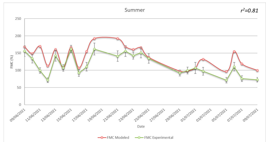
Figure 7. Temporal evolution of observed and predicted FMC for Cistus monspeliensis during summer conditions.
