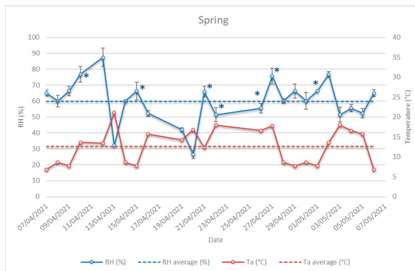
Figure 2. Meteorological data (Temperature and Relative Humidity) during spring conditions. Asterisks indicate days influenced by precipitation.
