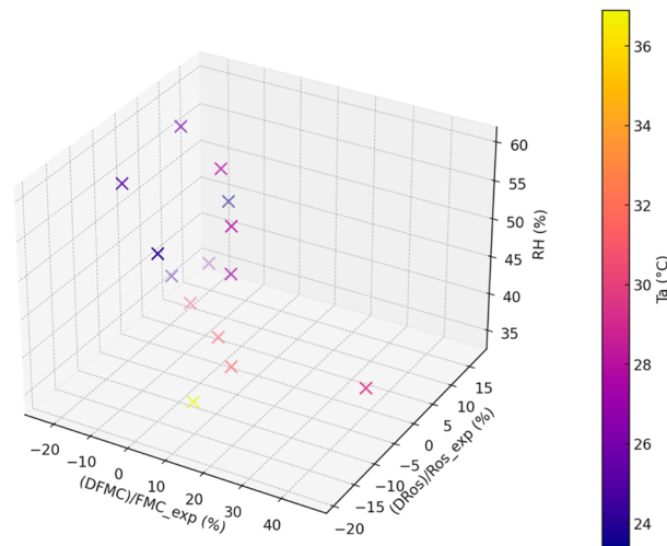
Figure 10. Regime-dependent distribution of DFMF/FMF_exp and DRoS/RoS_exp as a function of air temperature and relative humidity.
