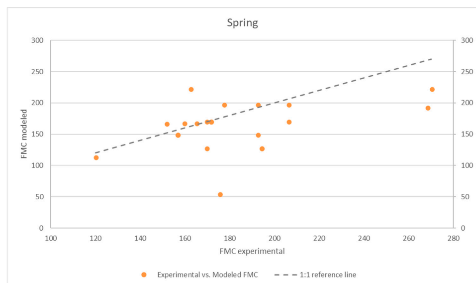
Figure 8. Experimental vs. modeled FMC for Cistus monspeliensis in spring conditions.
