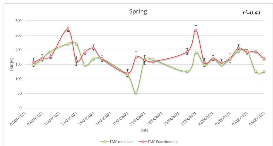
Figure 6. Temporal evolution of experimental and modeled FMC for Cistus monspeliensis during spring conditions.
