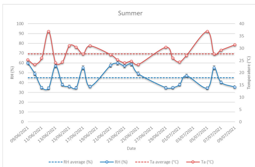
Figure 3. Meteorological data (Temperature and Relative Humidity) during summer conditions.
