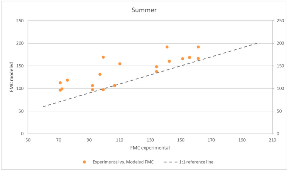
Figure 9. Experimental vs. modelled FMC for Cistus monspeliensis in summer conditions.
