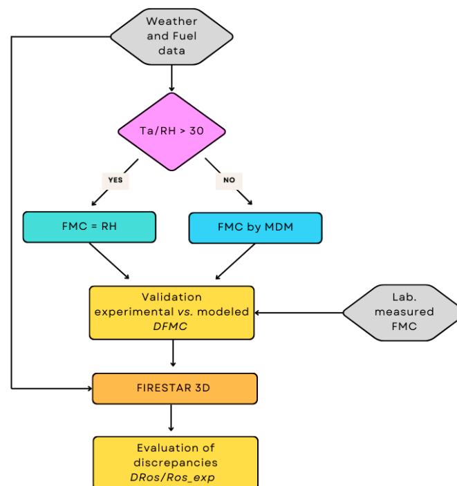
Figure 5. The empirical threshold condition applied to field data when T_a/RH > 30 .
