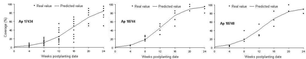
Figure 2. Dispersion data coverage and lines fixed to three-parameter sigmoid model, shown in Table 2.
