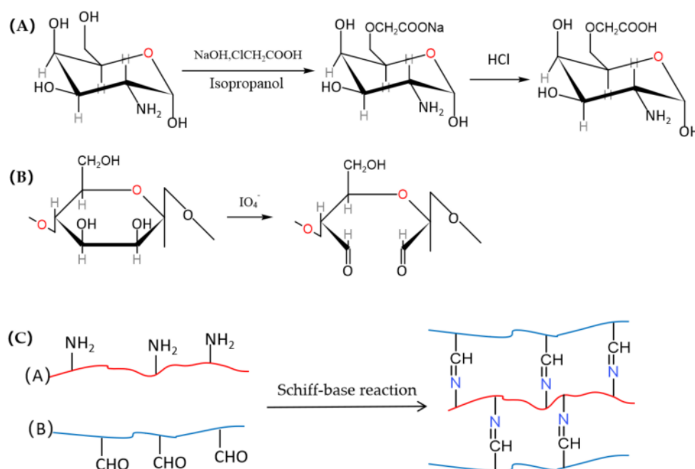
Figure 1. The schematic of O-CCS (A), OP (B), and OPHs (C), respectively.
