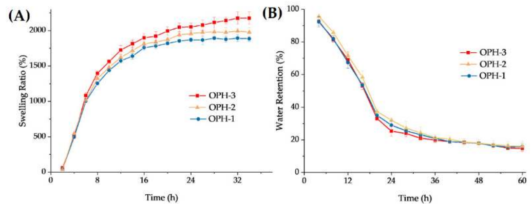
Figure 5. Swelling ratio (A) and water-retention ratio (B) of OPHs (mean \pm SD, n = 3 ).
