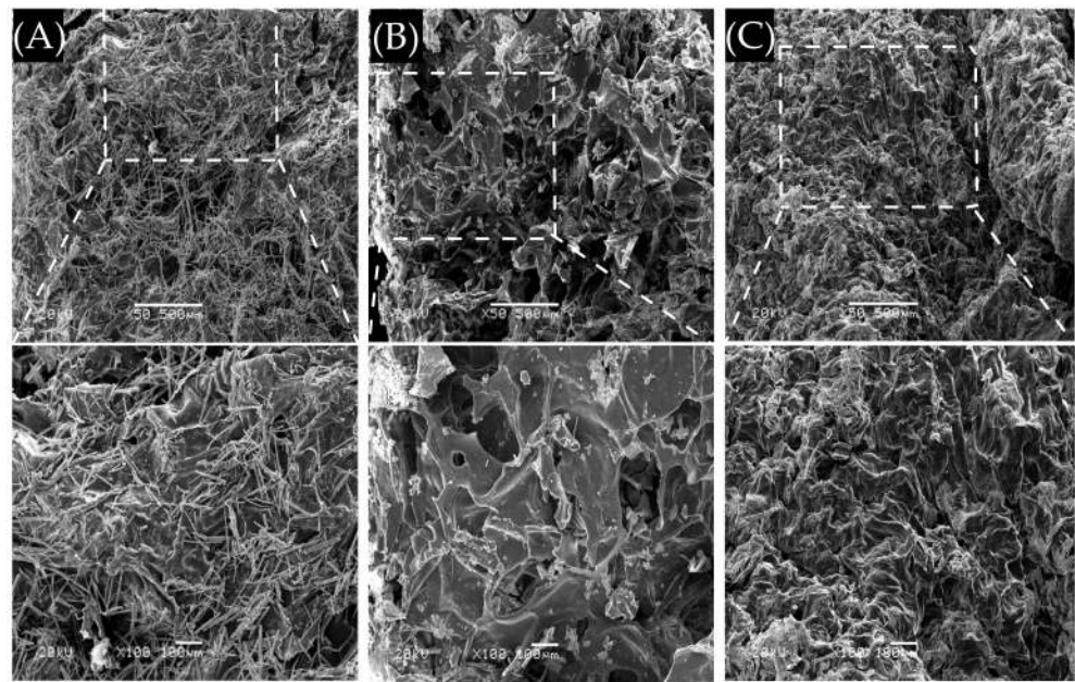
Figure 3. SEM images of the OPHs. (A–C) OPH-1, OPH-2, and OPH-3, respectively. They were magnified as multiples of 50 and 100, and the scales are 500 \mu\text{m} and 100 \mu\text{m} , respectively.
