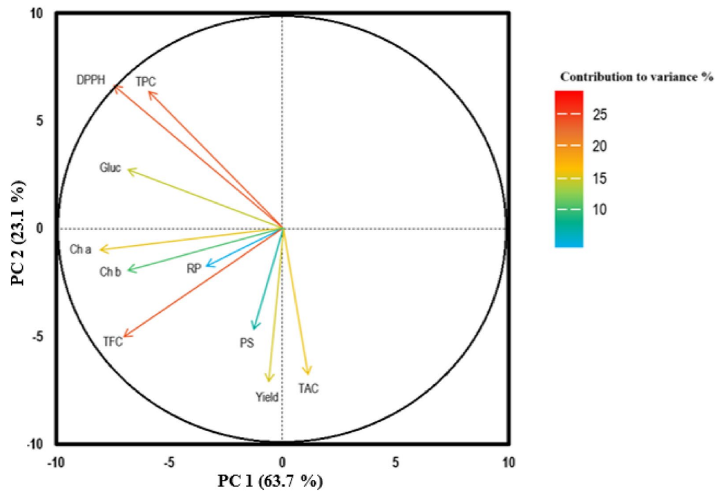
Fig. 4 Main Component Analysis (PCA) shows the correlations between antioxidant activities, the content of TPC, TFC, PS, carbohydrates, and Ch – a and Ch – b of different M. longifolia extracts
