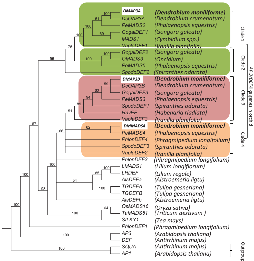
Fig. 2. The most parsimonious tree of AP3/DEF-like genes in plants based on an alignment of the full-length amino acid sequence using UPGMA method. Numbers are bootstrap values after 100 replicate runs. The four orchid AP3/DEF like clades were indicated by brackets. The B-class sequences isolated from D. moniliforme in this study were bolded. Two class A MADS-box genes were used as outgroup.
