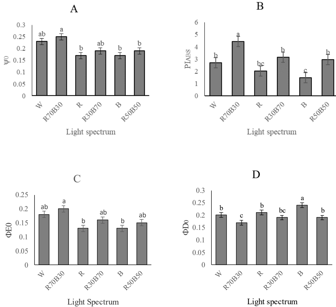
Fig. 5. A) Possibility that an electron travels further than QA ( \psi_0 ), B) performance index in light absorption basis ( PI_{ABS} ), C) quantum yield of electron transport ( \Phi_{E0} ), and D) Quantum yield of energy dissipation ( \Phi D_0 ) in the D. moldavica plants (DMRT, p \leq 0.05 )
