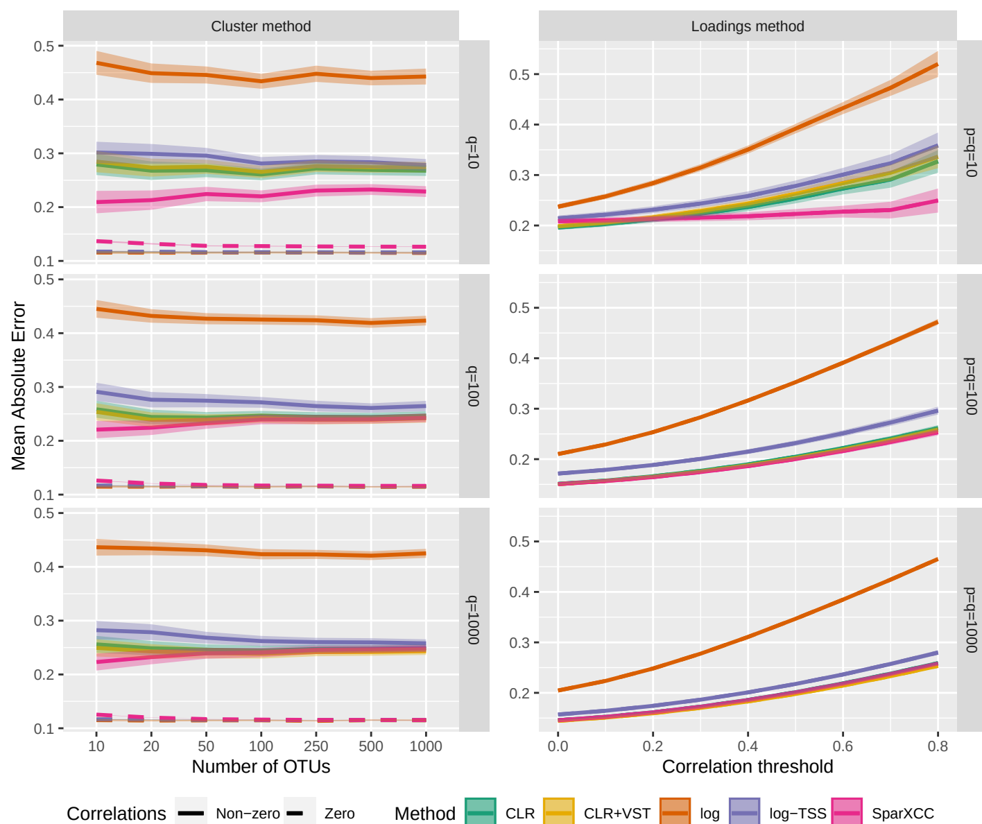
Fig 4. MAE of different cross-correlation methods for correlation matrices generated by the cluster method (left column) and the loadings method (right column) in case C. For the cluster method, different p (number of OTUs) and q (number of genes) are used. For the loadings method, threshold values t = 0, 0.1, \dots, 0.8 and different p and q are used. The lines show the mean accuracy, and the edges of the envelopes show \pm 1.96 standard errors (SE). The results are based on 500 simulated datasets where each simulated dataset has 50 replicates.
