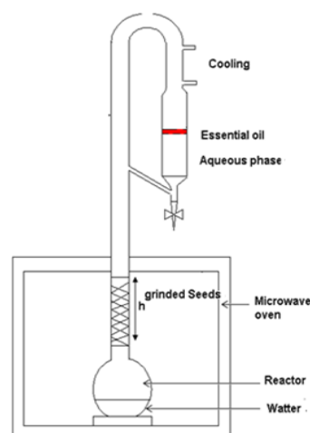
Fig. 1 Steam distillation assisted by microwave, seeds inside of oven apparatus SDAM
