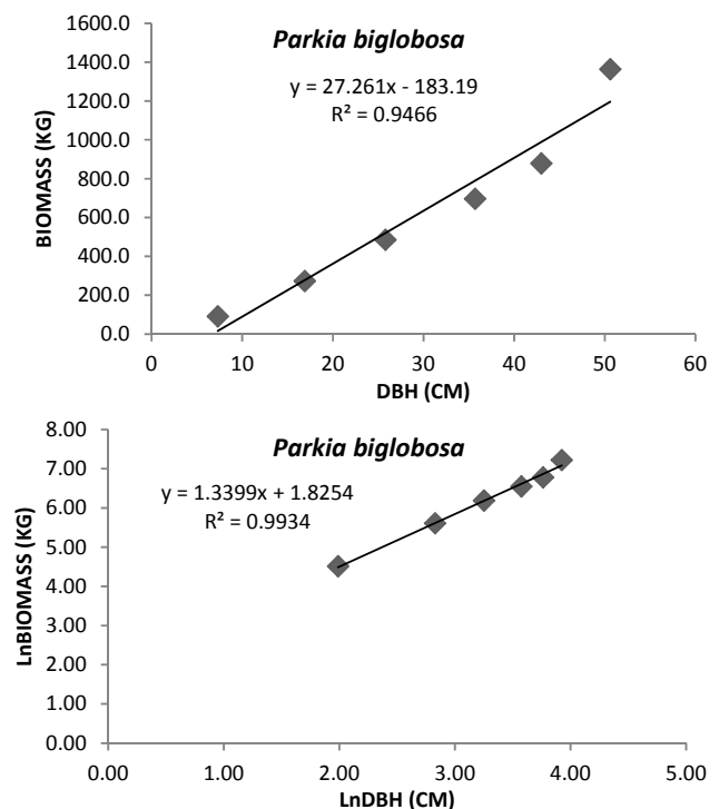
Fig. 10 Regression plots and line of best fit on raw data (top) and on logarithmic scale (bottom) for Parkia biglobosa species
