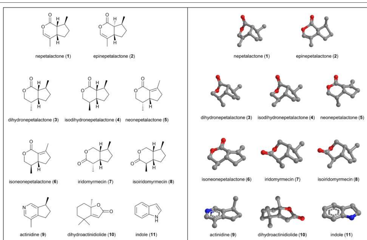
Fig. 13 Structures of the single compounds used for bioassays with domestic cats. Two dimensional structures are shown on the left, 3D structures are shown on the right. Oxygen atoms are shown in red, nitrogen in blue. Nepetalactone (1) and epinepetalactone (2) are also referred to as cis-trans -nepetalactone and trans-cis -nepetalactone, respectively. Note how the location of the carbonyl group is different between the type I lactones 7–8 and the type II lactones 1–6
