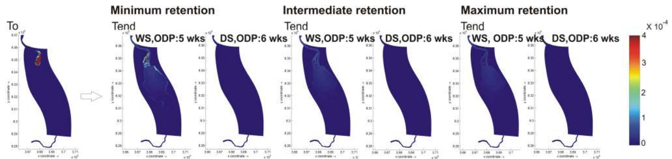
Fig. 5b. Results of scenario 1 (effect of species-specific buoyancy) showing the distribution plots of Ceriops tagal . WS = wet season, DS = dry season, ODP = obligated dispersal period. Red, yellow and light blue colours indicate a high, medium and low concentration of propagules respectively.
