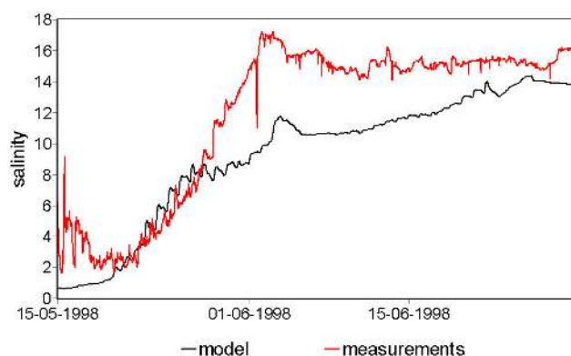
Fig. 3. Validation of the hydrodynamic model: presentation of the salinities measured in the field (red) versus the salinities generated by the model (black).
