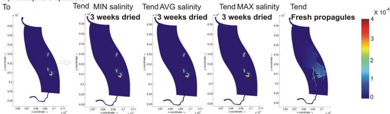
Fig. 6b. Results of scenario 2 (effect of drying) showing the distribution plots of Rhizophora apiculata in the dry season. Red, yellow and light blue colours indicate a high, medium and low concentration of propagules respectively.
