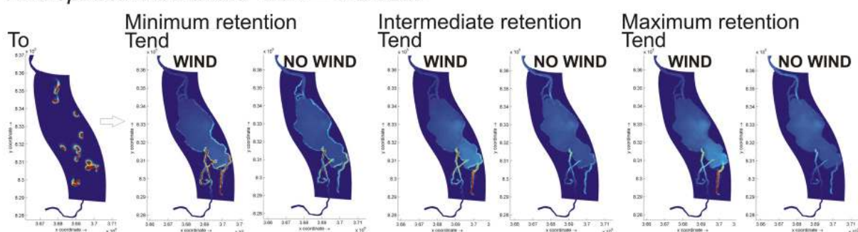
Fig. 7. Results of scenario 3 (the effect of “additional wind”) showing the distribution plots of propagules of Avicennia officinalis and Rhizophora mucronata . Scale is applicable to all distribution patterns. Red, yellow and light blue colours indicate a high, medium and low concentration of propagules respectively.
