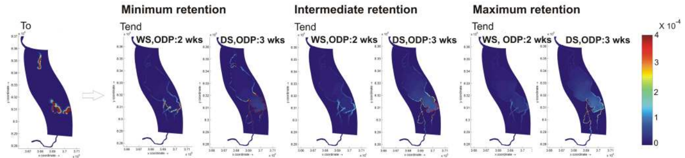
Fig. 5a. Results of scenario 1 (effect of species-specific buoyancy) showing the distribution plots of Avicennia officinalis . WS = wet season, DS = dry season, ODP = obligated dispersal period. Red, yellow and light blue colours indicate a high, medium and low concentration of propagules respectively.
