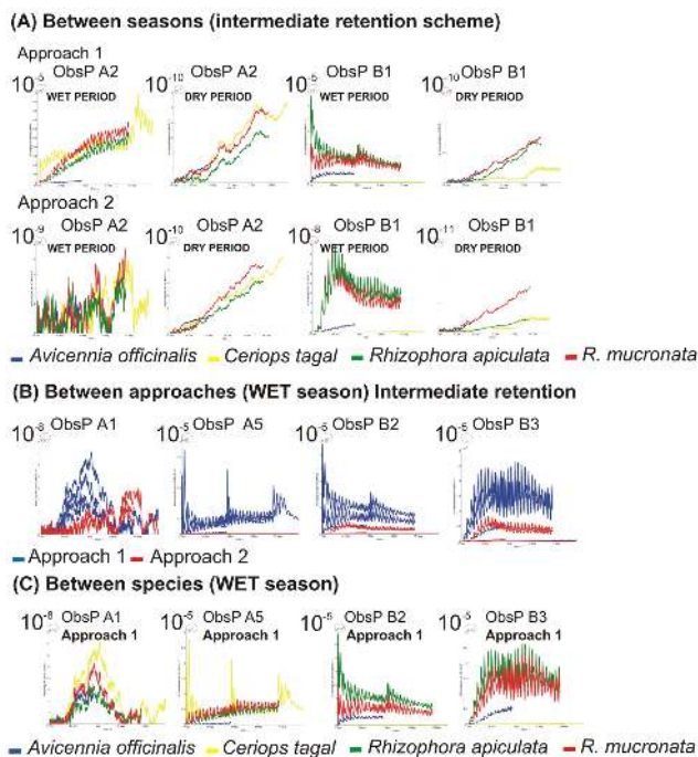
Fig. 8. Results of scenario 4 (the effect of dike removal) showing the time-series plots of Avicennia officinalis , Ceriops tagal and Rhizophora apiculata and Rhizophora mucronata . A comparison was made between (A) seasons (wet versus dry season), (B) approaches of outer dike removal (In approach 1, 60 m of an outer dike was removed at the northeastern side of shrimp farm A and the northern side of shrimp farm B, while in approach 2 part 60 m of the outer dike at the southeastern side of shrimp farm A and the north-western side of shrimp farm B was removed) and (C) the different species. ObsP Ax = observation point in shrimp farm area A, ObsP Bx = observation point in shrimp farm area B. X-axes = buoyancy period (days), y-axes = propagule density m -2 .
