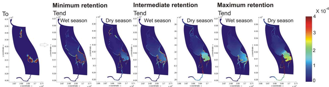
Fig. 4a. Results of the sensitivity analysis: distribution patterns for the species Avicennia officinalis when varying the retention schemes from minimum, intermediate to maximum retention values. Red, yellow and light blue colours indicate a high, medium and low concentration of propagules respectively.
